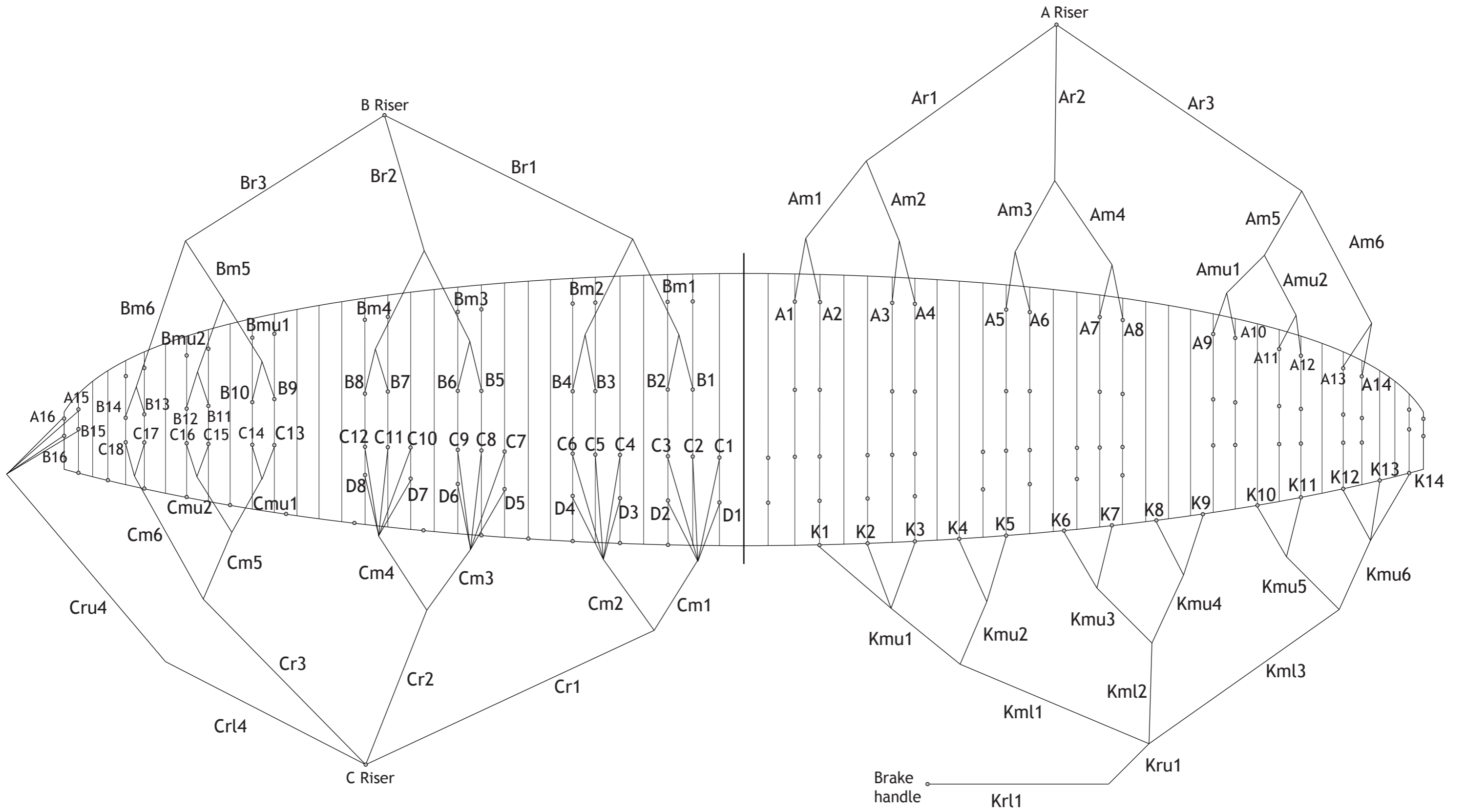
ALPINA2 Rigging Diagram
