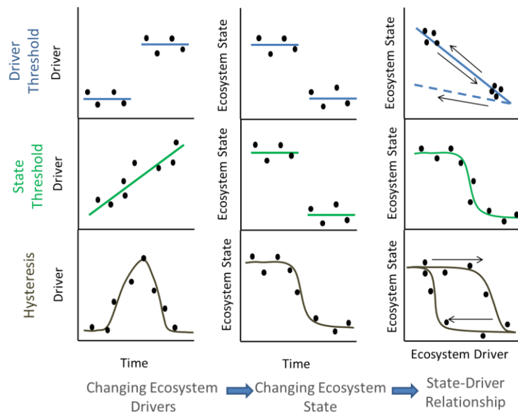
Fig 1. Three scenarios for regime shift involve jumps in drivers (top row), non-linear response of ecosystem state to drivers (middle), and different non-linear responses as driver increases & decreases (bottom). When a driver is reversed, ecosystem state may return to the initial state (solid line top right), return to initial state via an alternative pathway (bottom right), or exhibit a novel state-driver relationships (dashed line top right). Modified from Andersen et al 2009.
