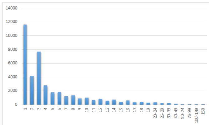
Fig. 1. Distribution of the number of worksheets over the spreadsheet files.
