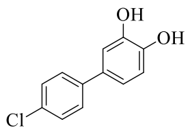
4-chloro-3',4'- dihydroxy-biphenyl
