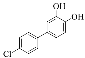
4-chloro-3',4'-dihydroxy-biphenyl
