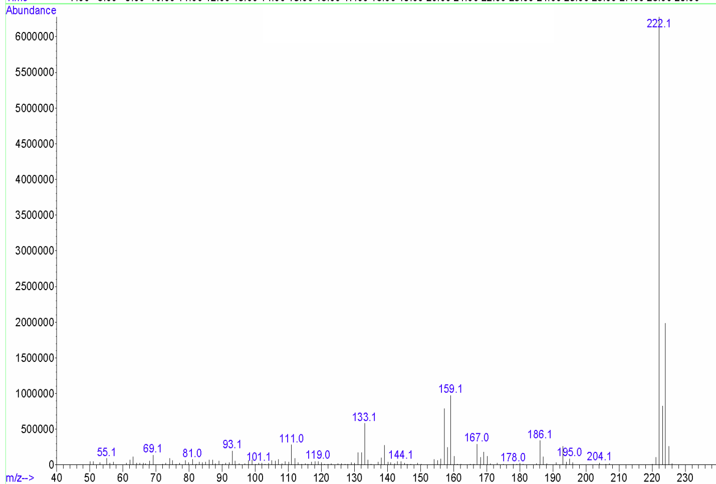
Gas chromatogram (top) and mass spectrum (bottom) of 4-chloro-3-fluoro-4'-hydroxy-biphenyl
