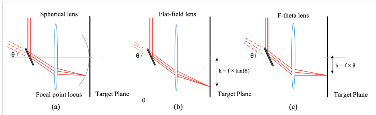
Fig. 11 – Types of lenses.
