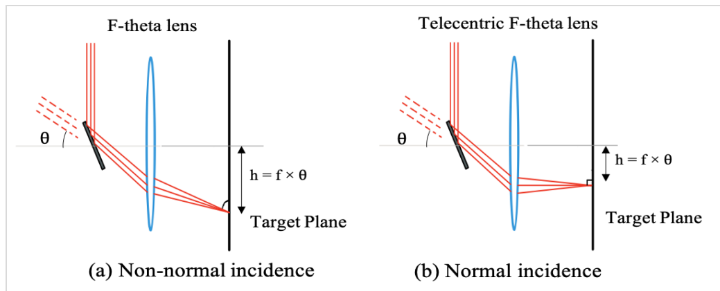
Fig. 12 – Types of f-theta lens.
