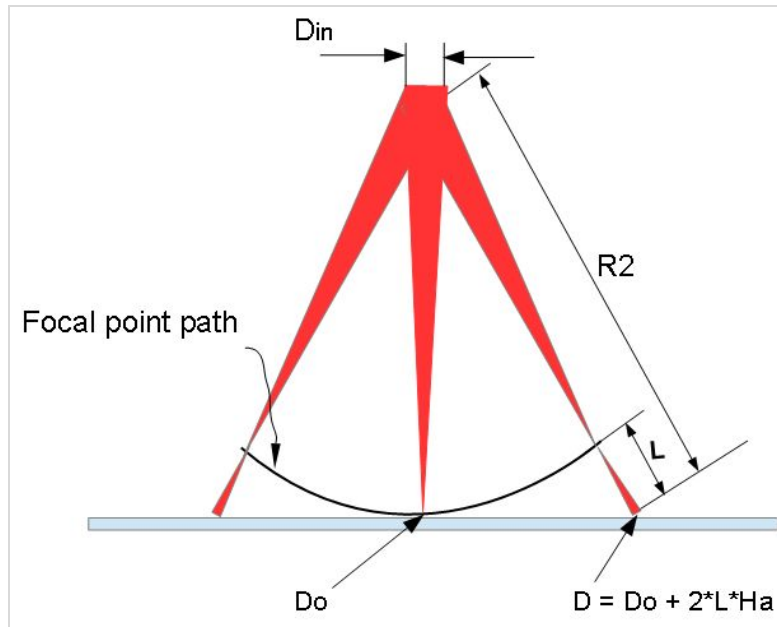
Fig. 5 – Schematic showing focal point path.
