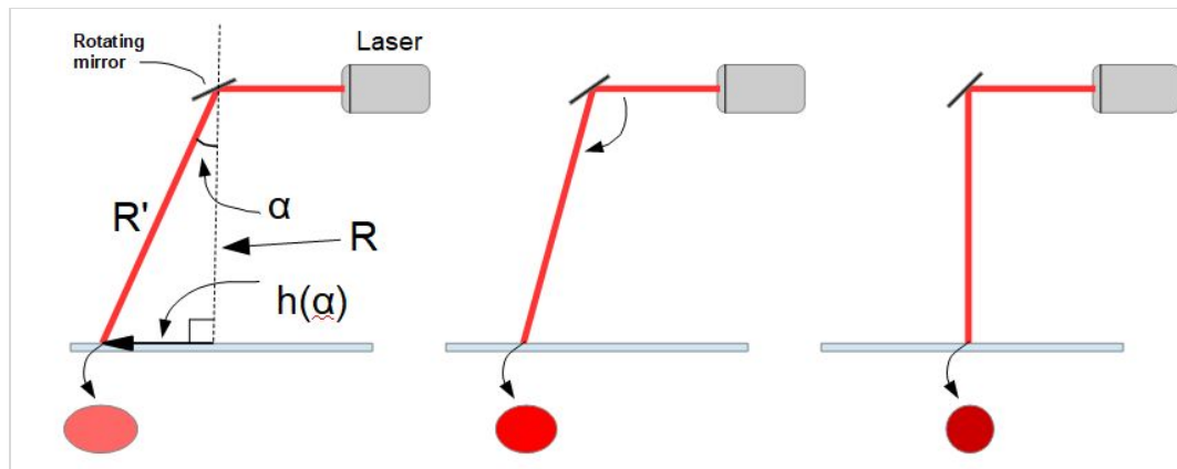
Fig 1. Schematic of a scanning system.
