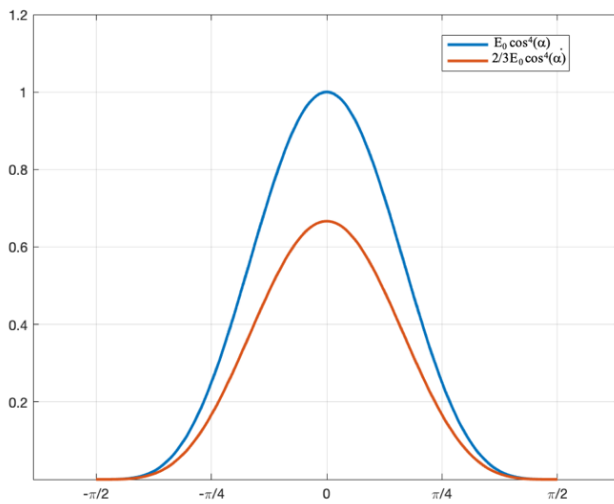
Fig. 9 – Plot for energy density for different OSC.
