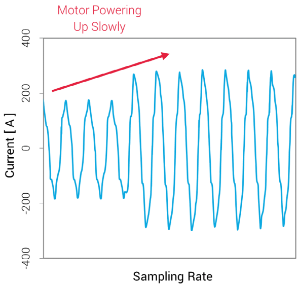
Figure 3: The network current before and after the motor powered up with a soft start setting (slowly).
