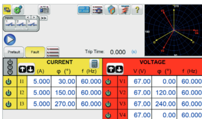
Figure 2: RTMS advanced user interface
