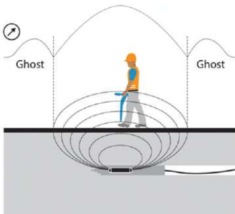
Figure 14.9 Locating a sonde
