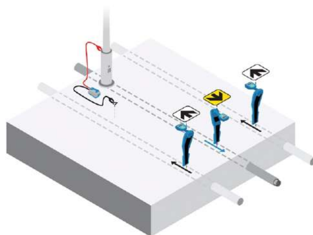
Figure 10.1: Current Direction
