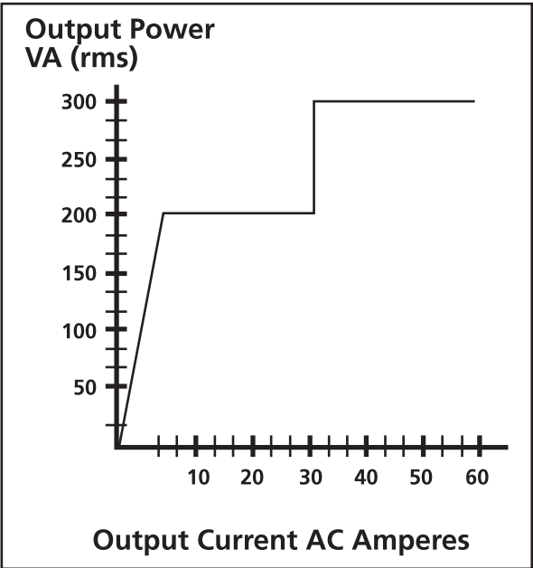
Current amplifier output power curve
