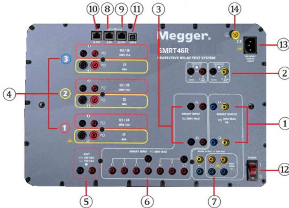
Figure 1 Top Panel SMRT46R (Pictured with Transducer Option)
