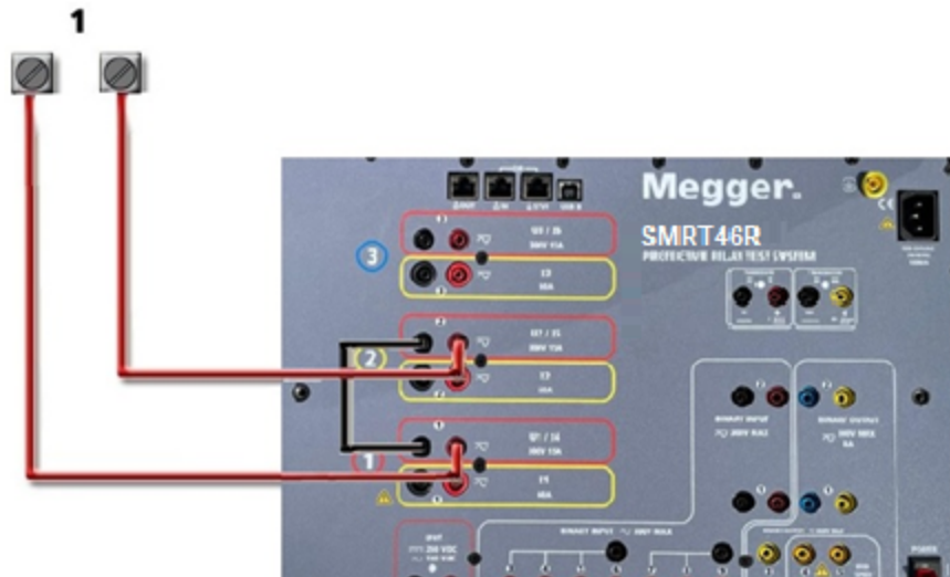
Figure 14 Series of Voltage Channels
