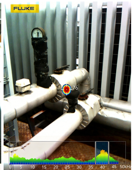
Leak detection on a pipeline
