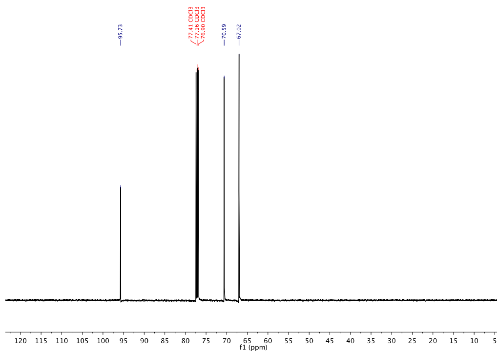
Figure S4. ^{13}\text{C} -NMR (125 MHz, \text{CDCl}_3 ) \delta 95.73, 70.59, 67.02 spectrum of poly(1,3,6-trioxocane). Signal at 77.16 ppm is residue \text{CHCl}_3 .
