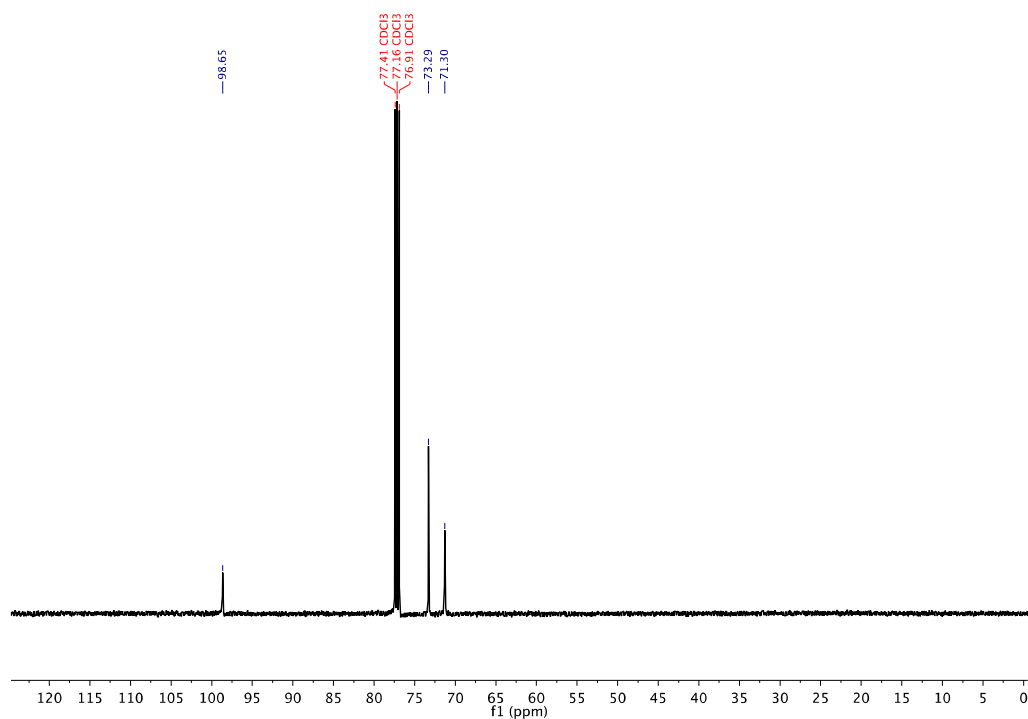
Figure S2. 13 C-NMR (125 MHz, CDCl 3 ) δ 98.65, 73.29, 71.30 spectrum of 1,3,6-trioxocane. Signal at 77.16 ppm is residue CHCl 3 .
