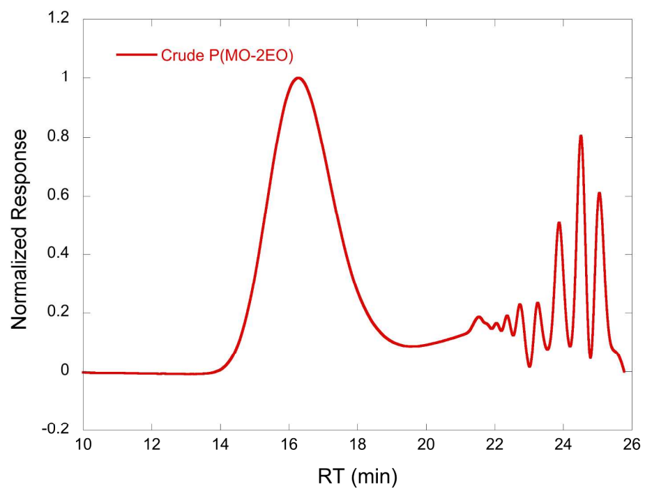
Figure S5. GPC traces of the crude mixture of Table 1 entry 3.
