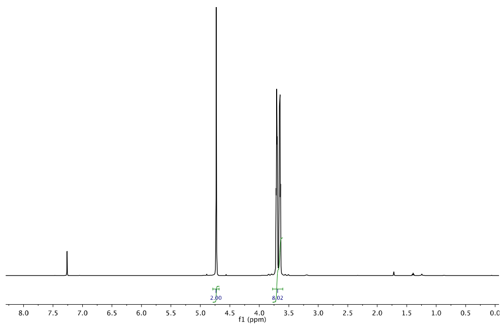
Figure S3. 1 H-NMR (500 MHz, CDCl 3 ) δ 4.73 (s, 2H), 3.74 – 3.61 (m, 8H) spectrum of poly(1,3,6-trioxocane). Signal at 7.26 ppm is residue CHCl 3 .
