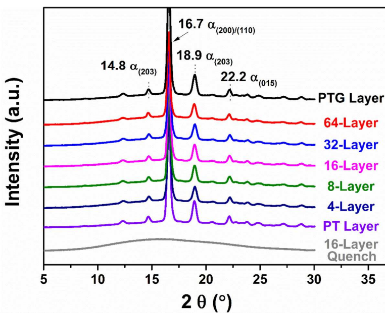
Figure S2. 1D-WAXD intensity profiles extracted from 2D-WAXD. The peak position and corresponding assignment to the specific lattice planes are marked on the diffraction peaks
