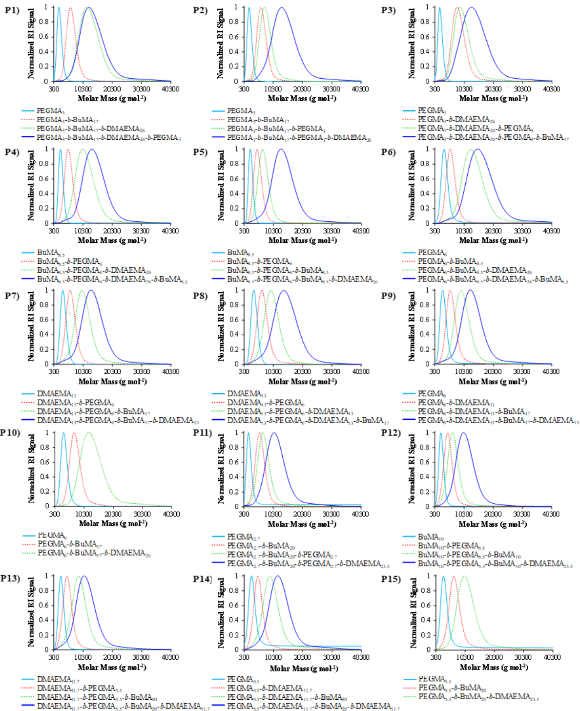
Figure S1. GPC chromatograms of the tetrablock terpolymers (P1-P9 and P11-P14), the triblock terpolymers (P10 and P15), and their liner precursors. The GPC chromatograms of the homopolymer, diblock, triblock, and tetrablock (if there is) are shown in light blue solid, red dotted, green dotted, and blue solid lines, respectively.
