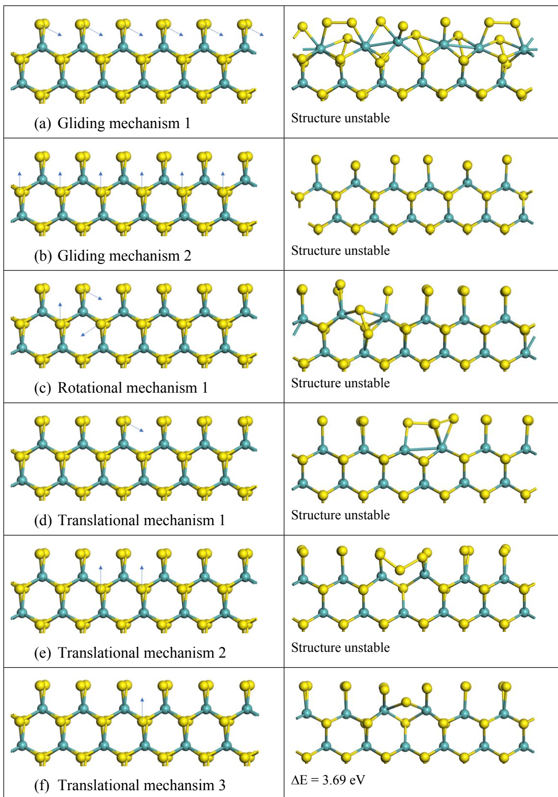
Figure S1. Calculated phase transition mechanisms for the Mo edge with 100%S.
