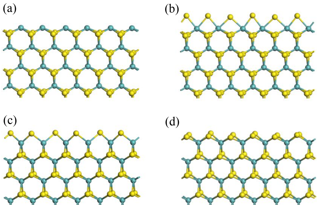
Figure S2. Optimized edges of 2H-MoS 2 . (a) Mo-edge with 0% S coverage; (b) Mo-edge with 50% S coverage; (c) S-edge with 50% S coverage; (d) S-edge with 100% S coverage.
