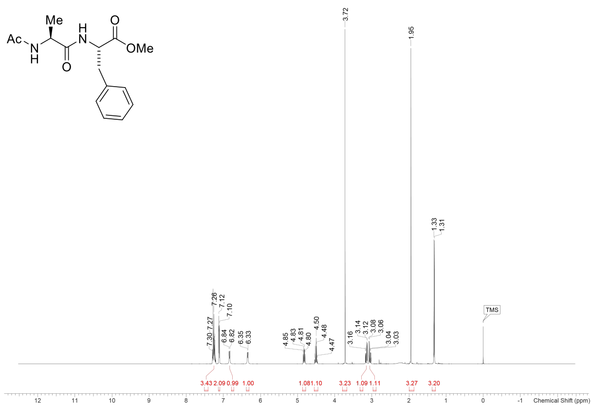
^1\text{H} NMR spectrum (400 MHz, \text{CDCl}_3 ) of 4a
