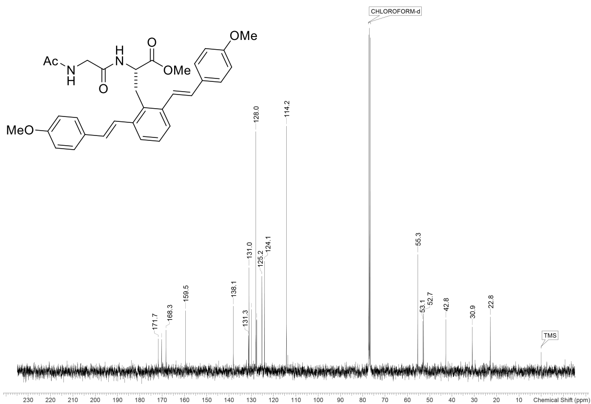
^{13}\text{C}\{^1\text{H}\} NMR spectrum (100 MHz, \text{CDCl}_3 ) of 3e
