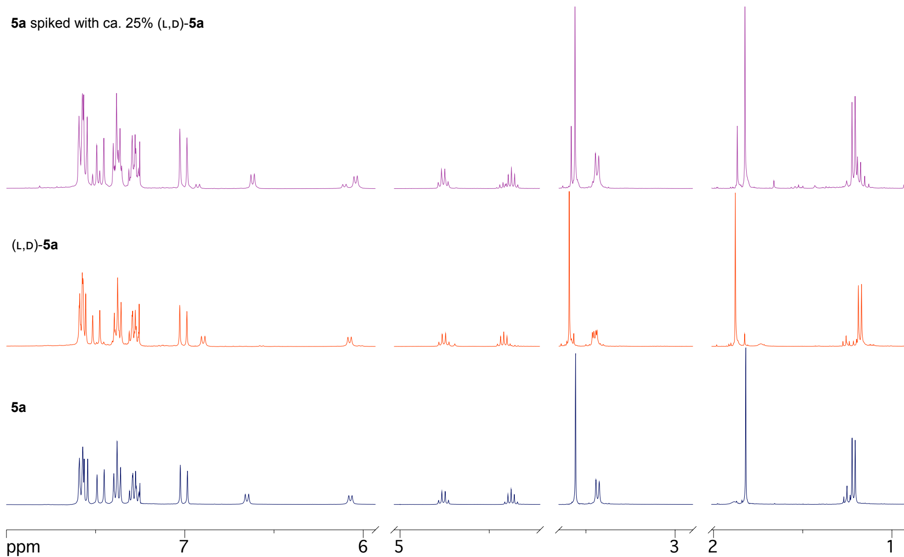
Figure S1. Comparison of 1 H NMR spectra for the modified peptides 5a and (L,D)- 5a . Complete spectra are presented in section 3 .
