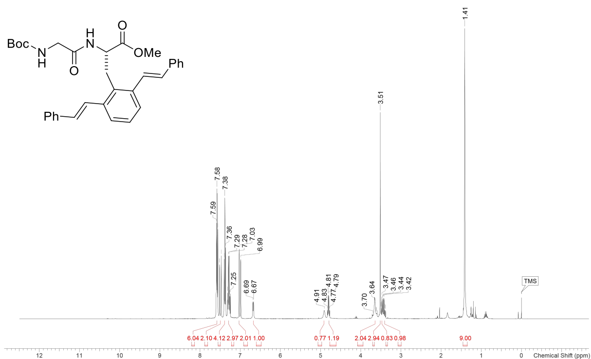
^1\text{H} NMR spectrum (400 MHz, \text{CDCl}_3 ) of 2b
