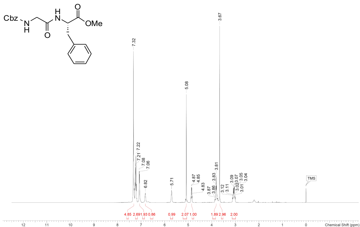
^1\text{H} NMR spectrum (400 MHz, \text{CDCl}_3 ) of 1d
