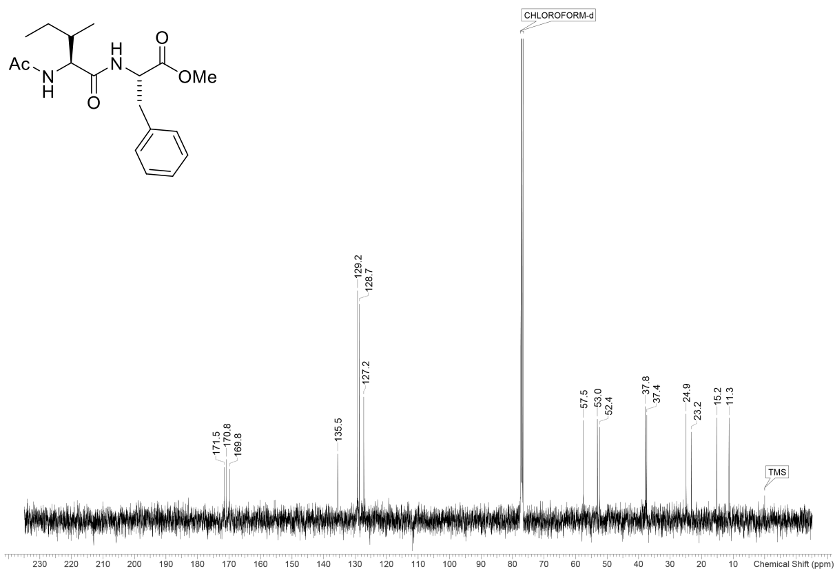
^{13}\text{C}\{^1\text{H}\} NMR spectrum (100 MHz, \text{CDCl}_3 ) of 4c
