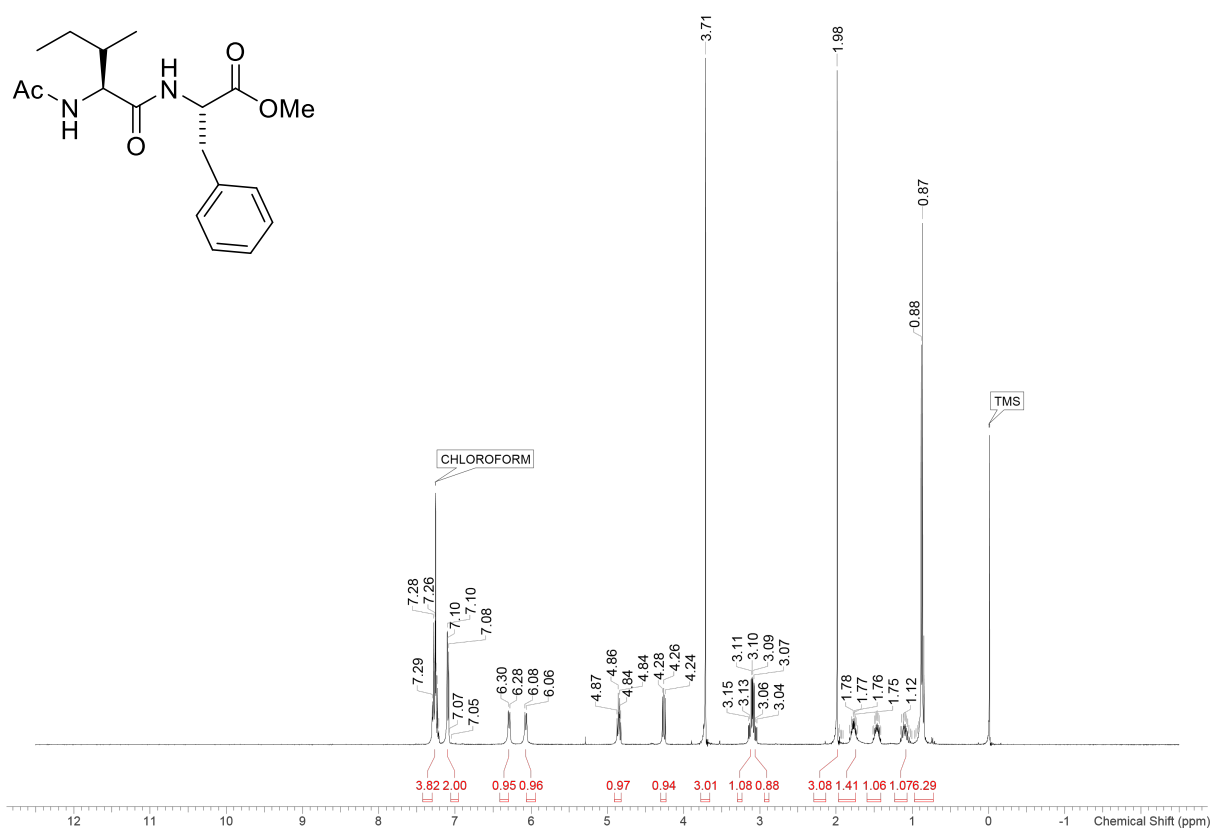
^{13}\text{C}\{^1\text{H}\} NMR spectrum (100 MHz, \text{CDCl}_3 ) of 4c
