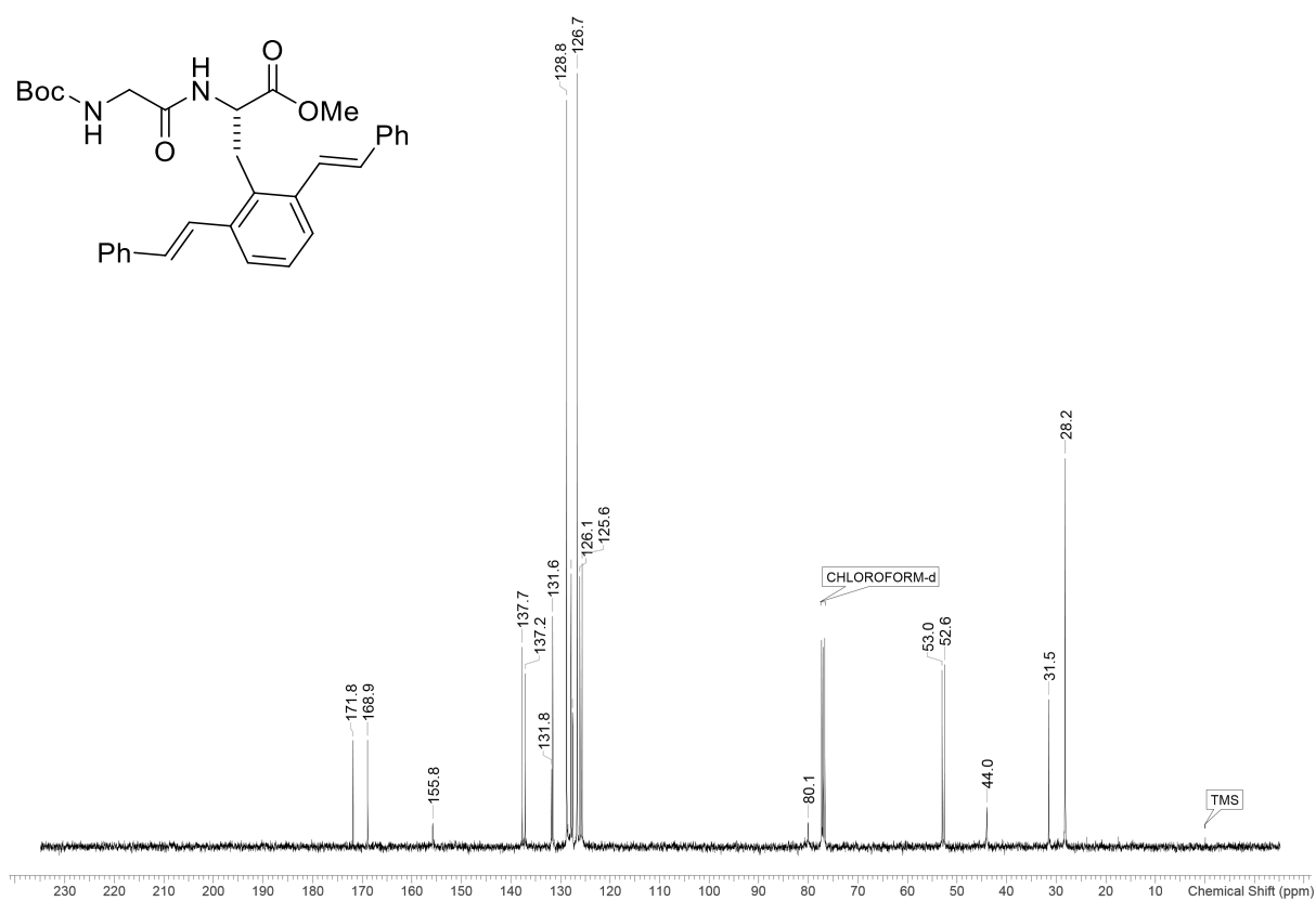
^{13}\text{C}\{^1\text{H}\} NMR spectrum (100 MHz, \text{CDCl}_3 ) of 2b
