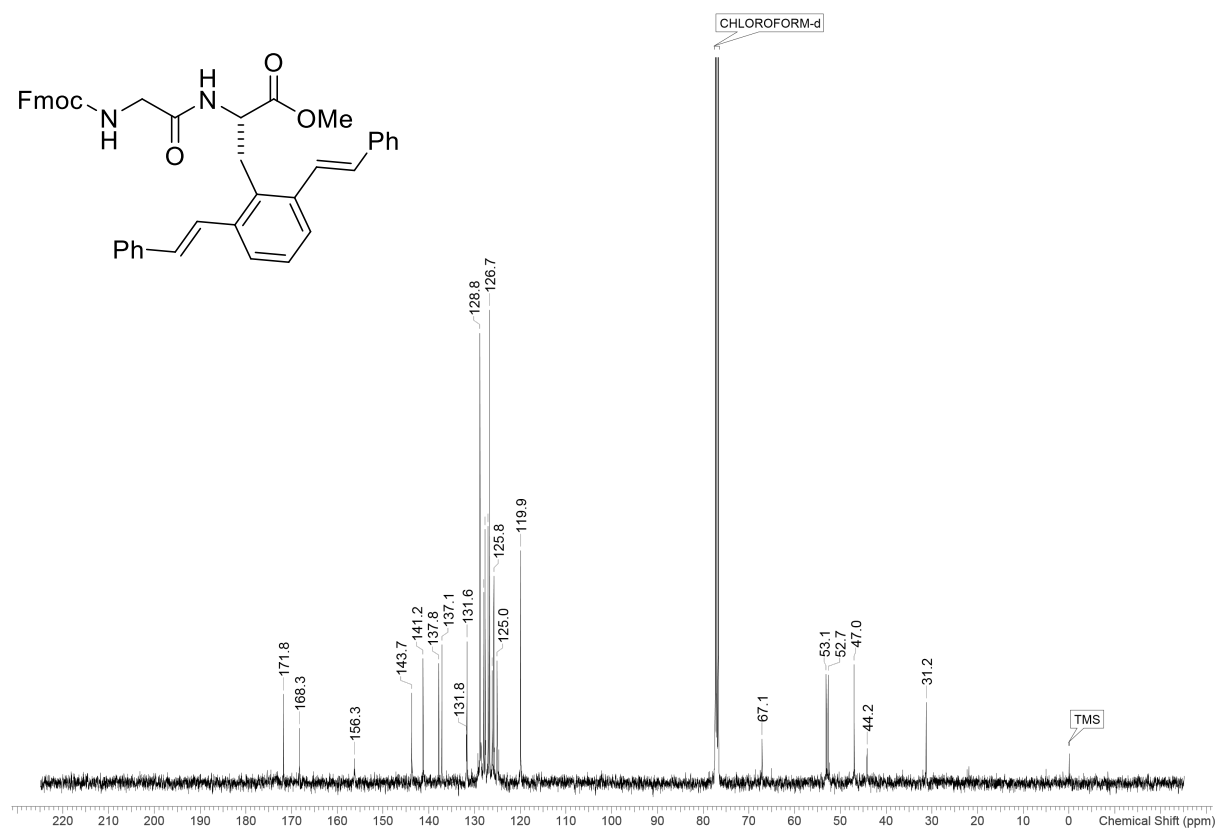
^{13}\text{C}\{^1\text{H}\} NMR spectrum (100 MHz, \text{CDCl}_3 ) of 2c
