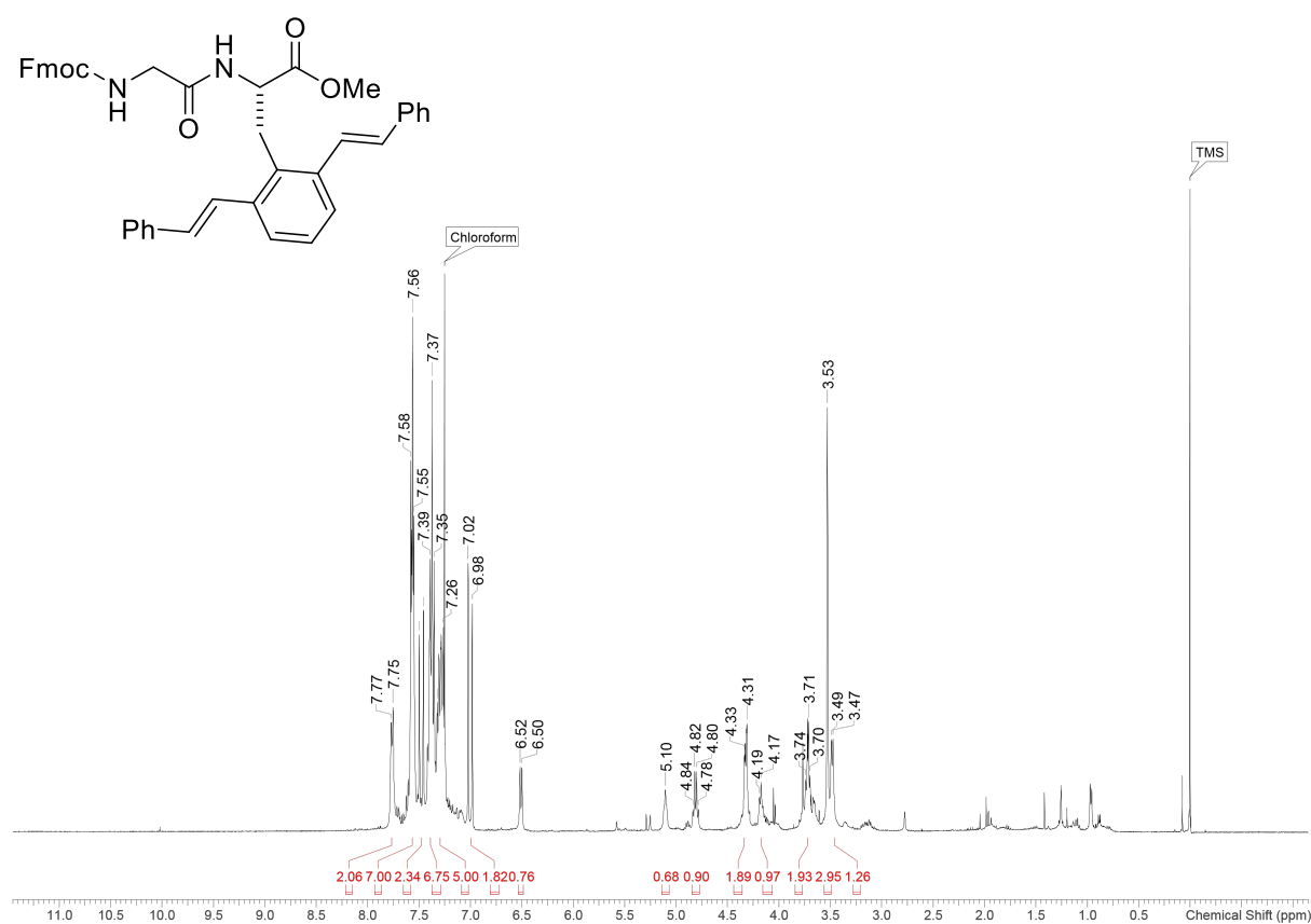
^1\text{H} NMR spectrum (400 MHz, \text{CDCl}_3 ) of 2c
