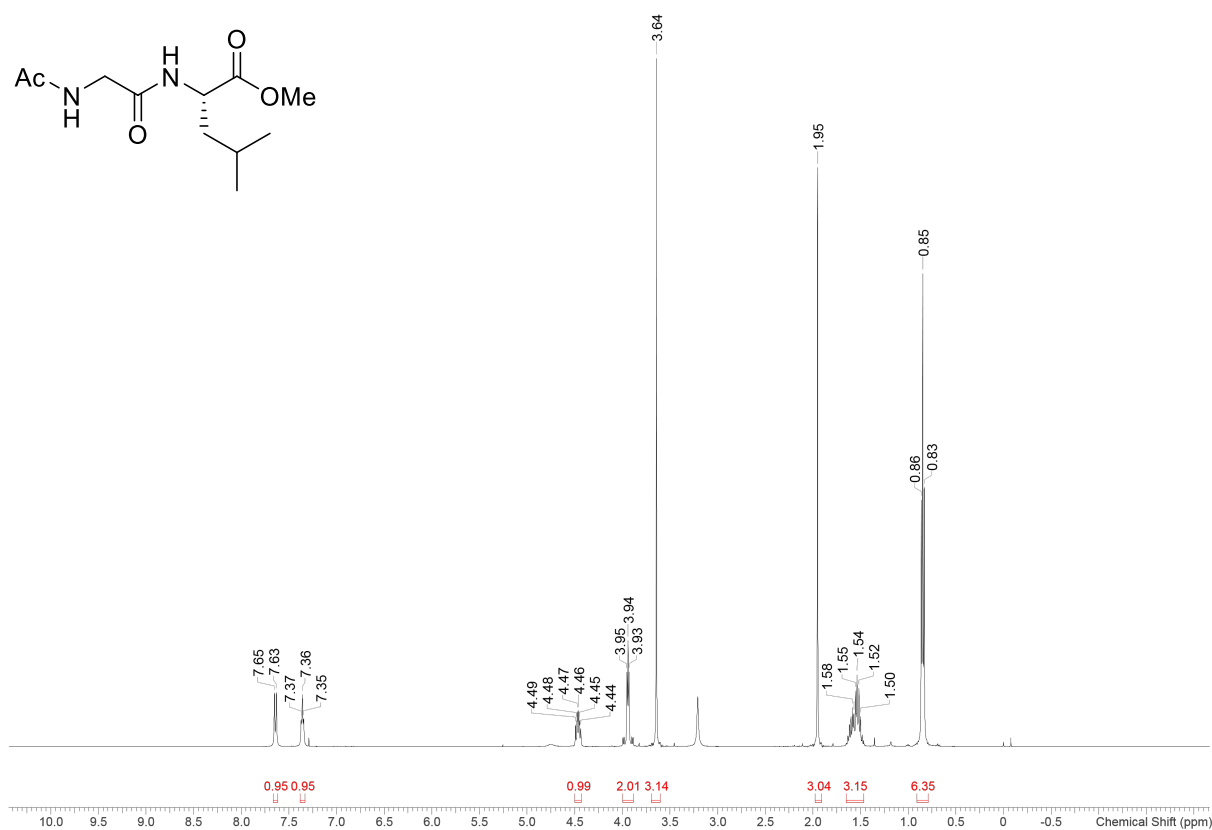
^{13}\text{C}\{^1\text{H}\} NMR spectrum (100 MHz, \text{CDCl}_3 ) of 4j
