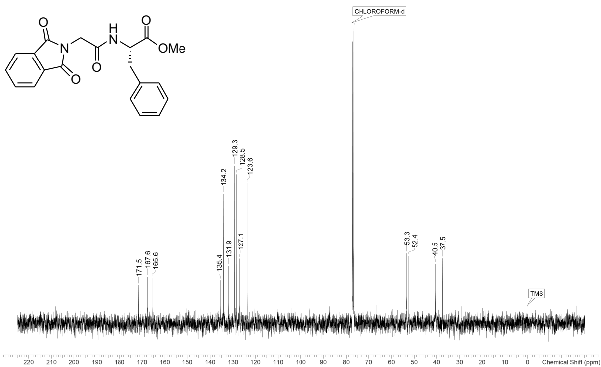
^{13}\text{C}\{^1\text{H}\} NMR spectrum (100 MHz, \text{CDCl}_3 ) of 1e
