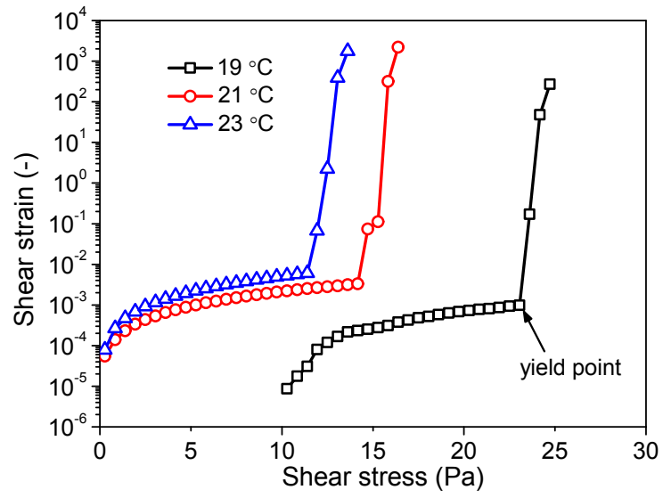
Figure S1. Evolution of the shear strain with the shear stress and the yield point of the waxy crude oil without scCO 2 treatment.
