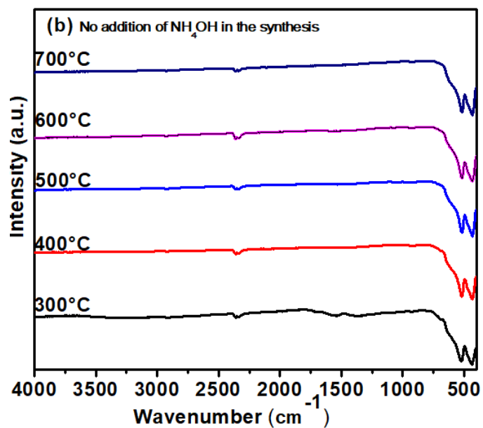
Figure S2. FTIR measurements of the \alpha -Fe 2 O 3 samples without the addition of ammonia in the synthesis.
