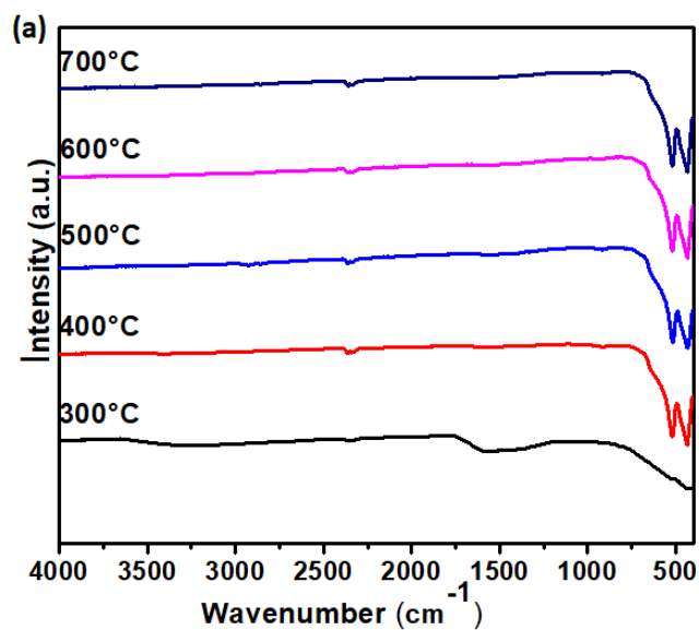
Figure S1. FTIR measurements of the \alpha -Fe 2 O 3 samples with the addition of ammonia in the synthesis.
