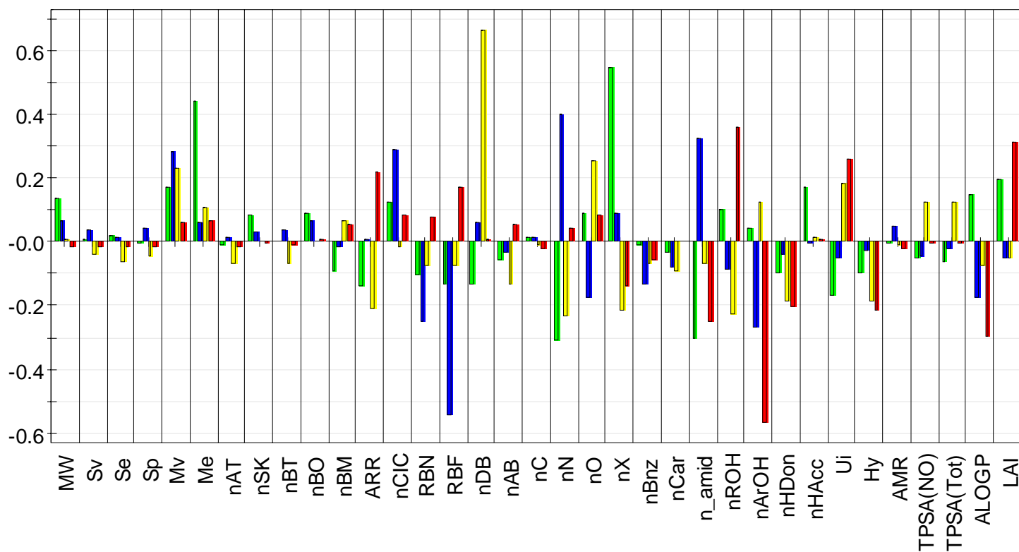
Supplementary Figure S1. Interpretation of PC5-PC8. Loading for each of the 35 descriptors in PC5 (green), PC6 (blue), PC7 (yellow), and PC8 (red). The Y-axis denotes loading and the X-axis gives the molecular descriptors.
