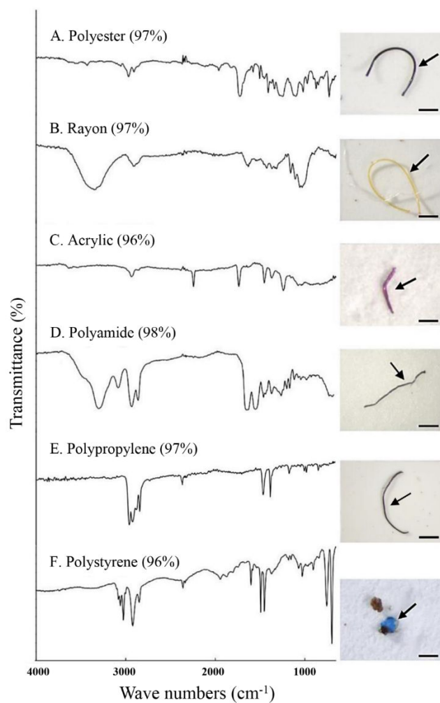
Figure S1. Analysis of microplastics with \mu -FTIR. The value in the brackets indicates the matches of the spectra with the standards. The black arrows in the photographs indicate the particles that were identified. Scale bar = 0.1 mm.
