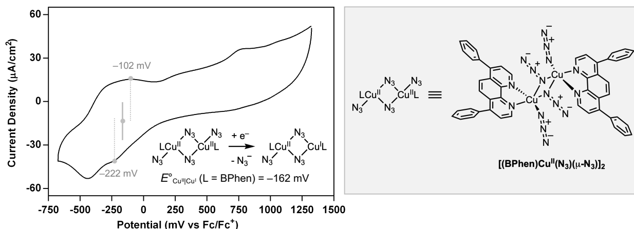
Figure S8. Cyclic voltammogram of [(\text{BPhen})\text{Cu}^{\text{II}}(\text{N}_3)(\mu\text{-N}_3)]_2 .
