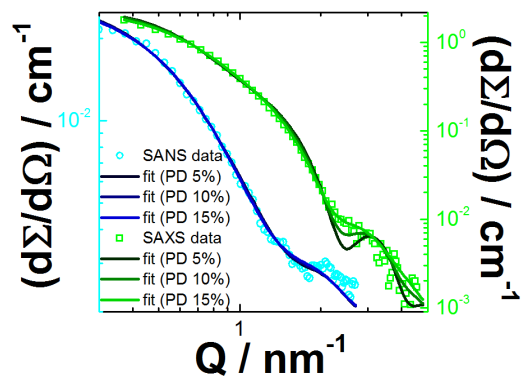
Figure S2: Comparison of different polydispersities for the main fraction shown for sample C.
