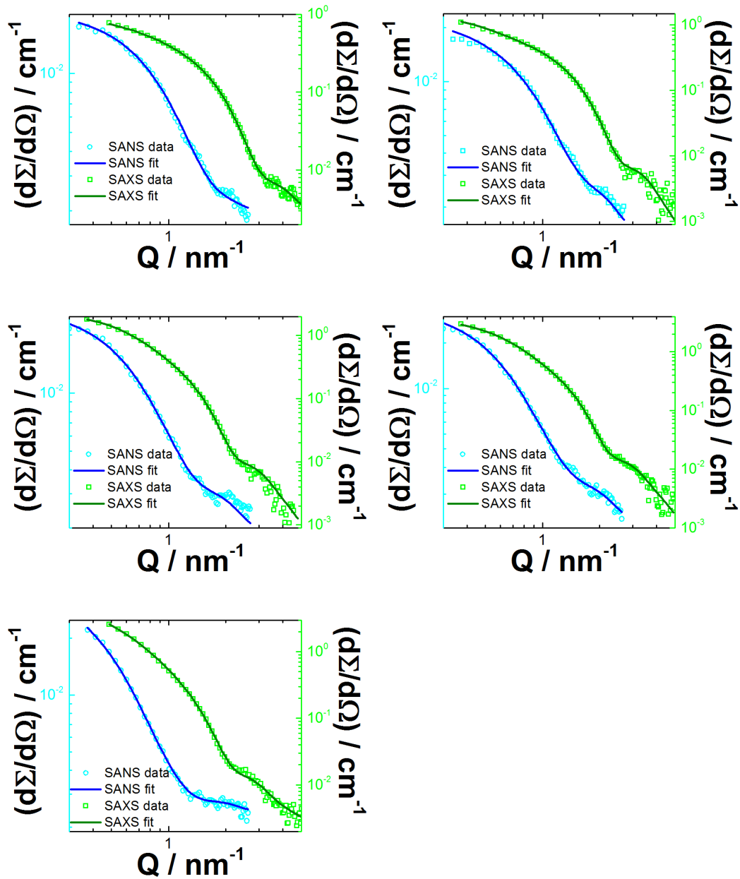
Figure S1: SAXS and SANS pattern of sample A (top left), B (top right), C (middle left), D (middle right) and sample E (bottom). The data is shown in a way that the complete extension of the different pattern can be seen.
