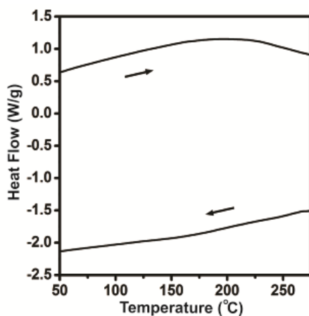
Figure S2. A heating and cooling DSC cycle on silver prepared via the thermal decomposition of silver benzoate.
