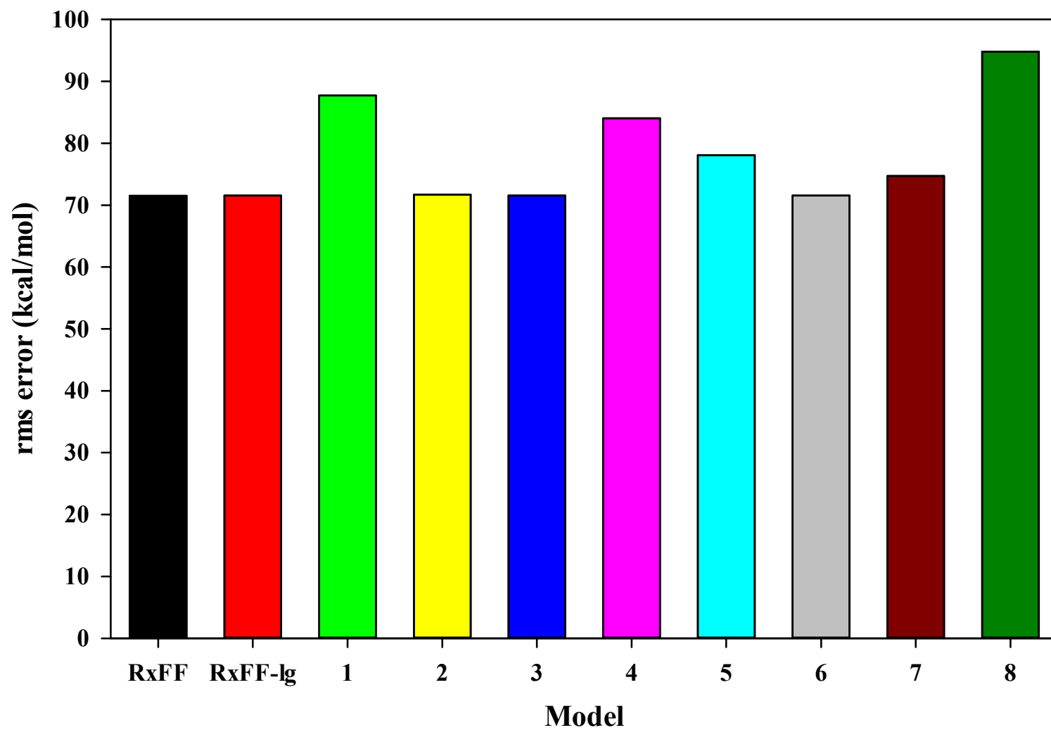
Fig. S1. Rms deviation from reference data for the ReaxFF, ReaxFF- lg and eight MOES models.
