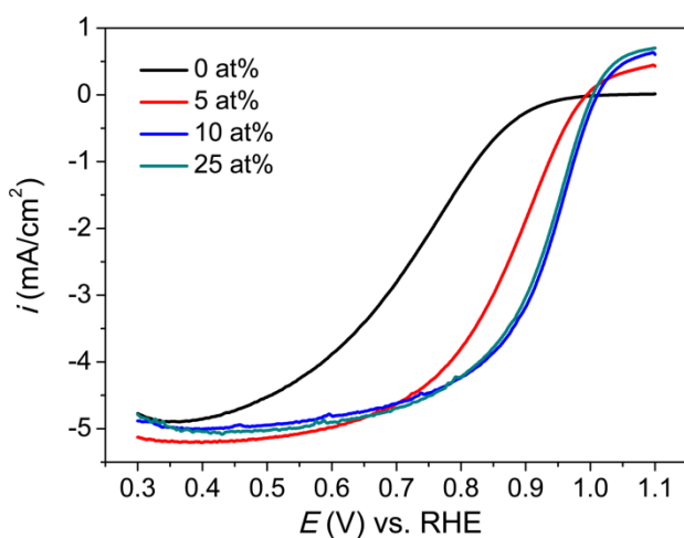
Figure S1. ORR polarization curves of Pt@Nb-TiO 2 catalysts with different amounts of Nb in the ceramic fibers.
