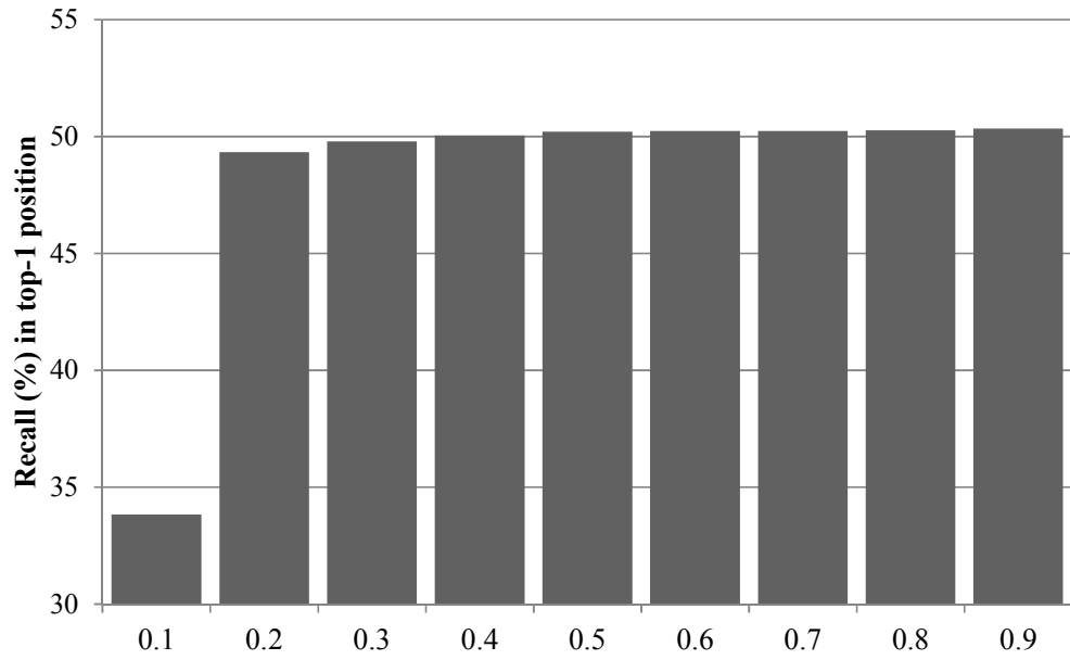
Figure S1. Recall of True Positives (TP) classes in the top-1 position as a function of the kernel smoothing parameter. Parameter h=0.9 was found to be optimum for this dataset.
