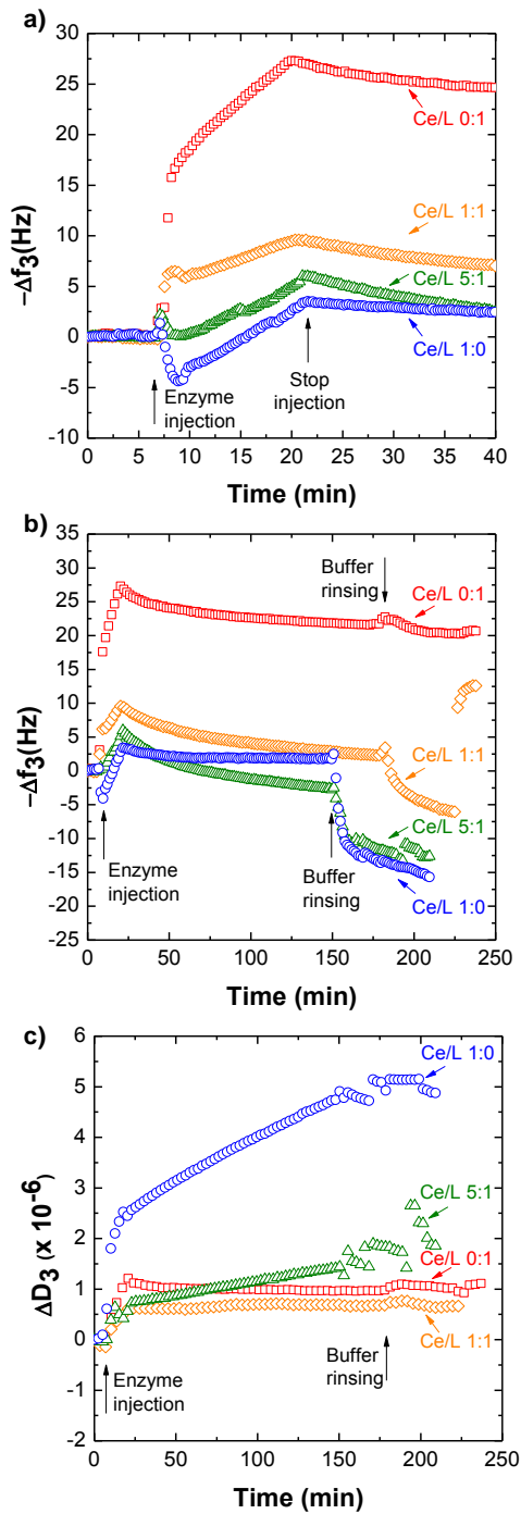
Figure S5. Negative shift in QCM frequency and changes in dissipation as a function of time after 15 minutes of continuous injection of an endoglucanase EG I (4,5 \mu\text{M} , flow rate of 100 \mu\text{l}/\text{min} ) followed by buffer (pH 5) rinsing as indicated by the vertical arrows. Profiles in (a) and (b) show the change in frequency for the first 40 minutes and the full time range (240) respectively. Data in panel (c) indicate the dissipation shift in the full time range.
