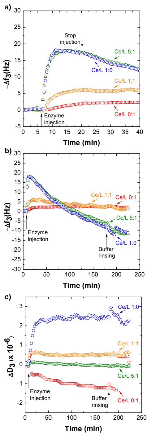
Figure S4. Negative shift in QCM frequency and changes in dissipation as a function of time after 15 minutes of continuous injection of a cellobiohydrolase CBH I core (4,5 \mu\text{M} , flow rate of 100 \mu\text{l}/\text{min} ) following by buffer (pH 5) rinsing as indicated by the vertical arrows. Profiles in (a) and (b) show the change in frequency for the first 40 minutes and the full time range (240 min) respectively. Data in panel (c) indicate the dissipation shift in the full time range.
