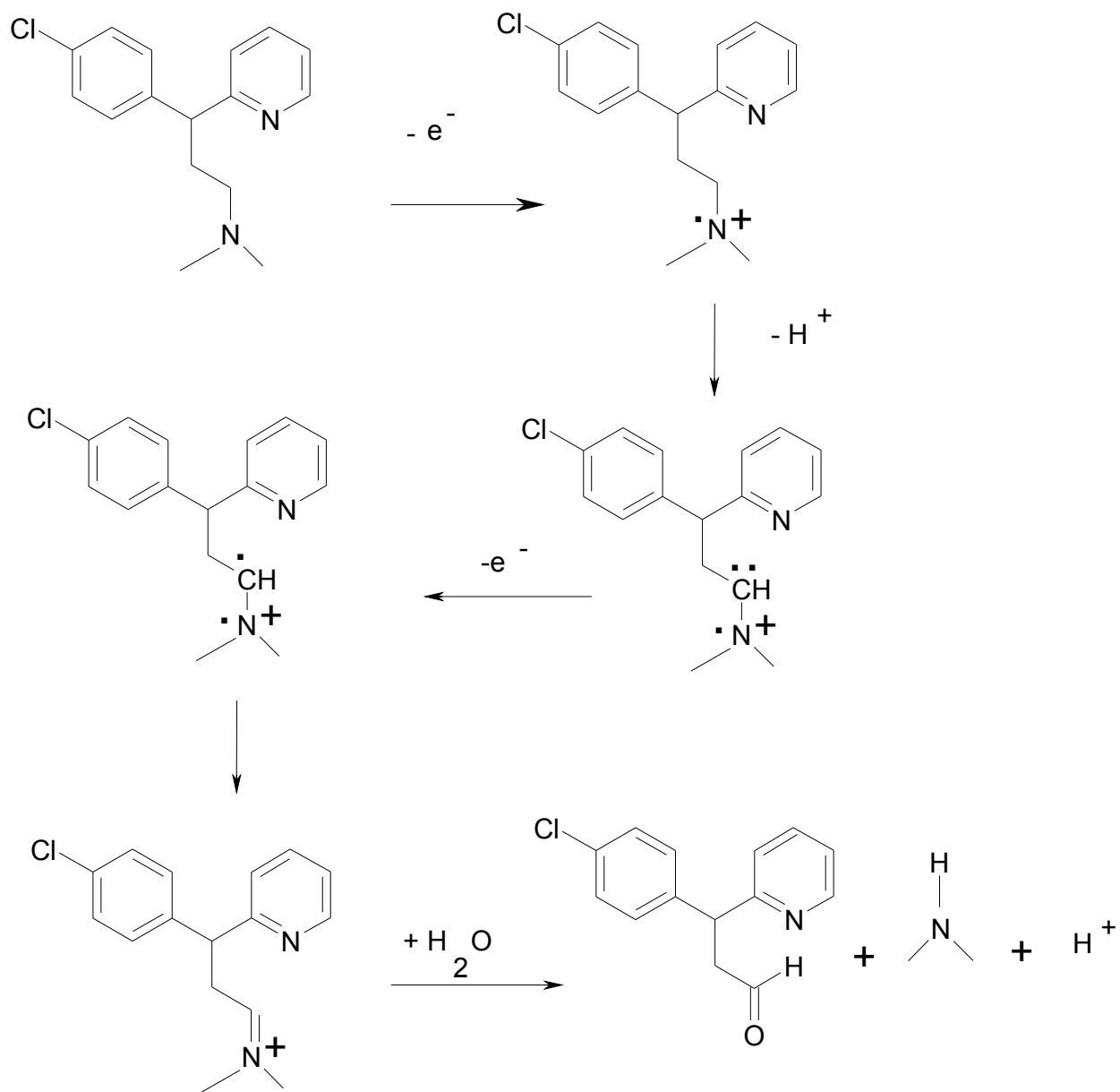
Scheme 1. Electrooxidation Mechanism of chlorpheniramine
