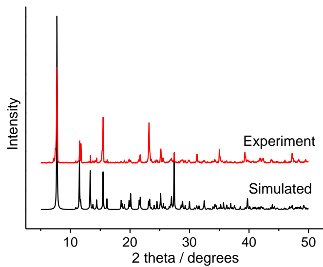
Figure S3. Simulated and experimental XRD powder patterns for 3 .
