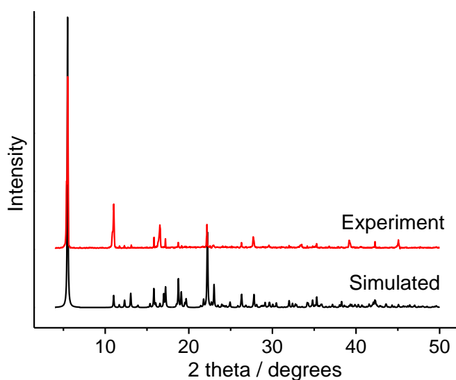
Figure S2. Simulated and experimental XRD powder patterns for 2 .
