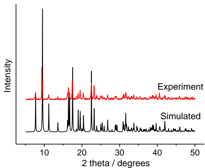
Figure S1. Simulated and experimental XRD powder patterns for 1 .
