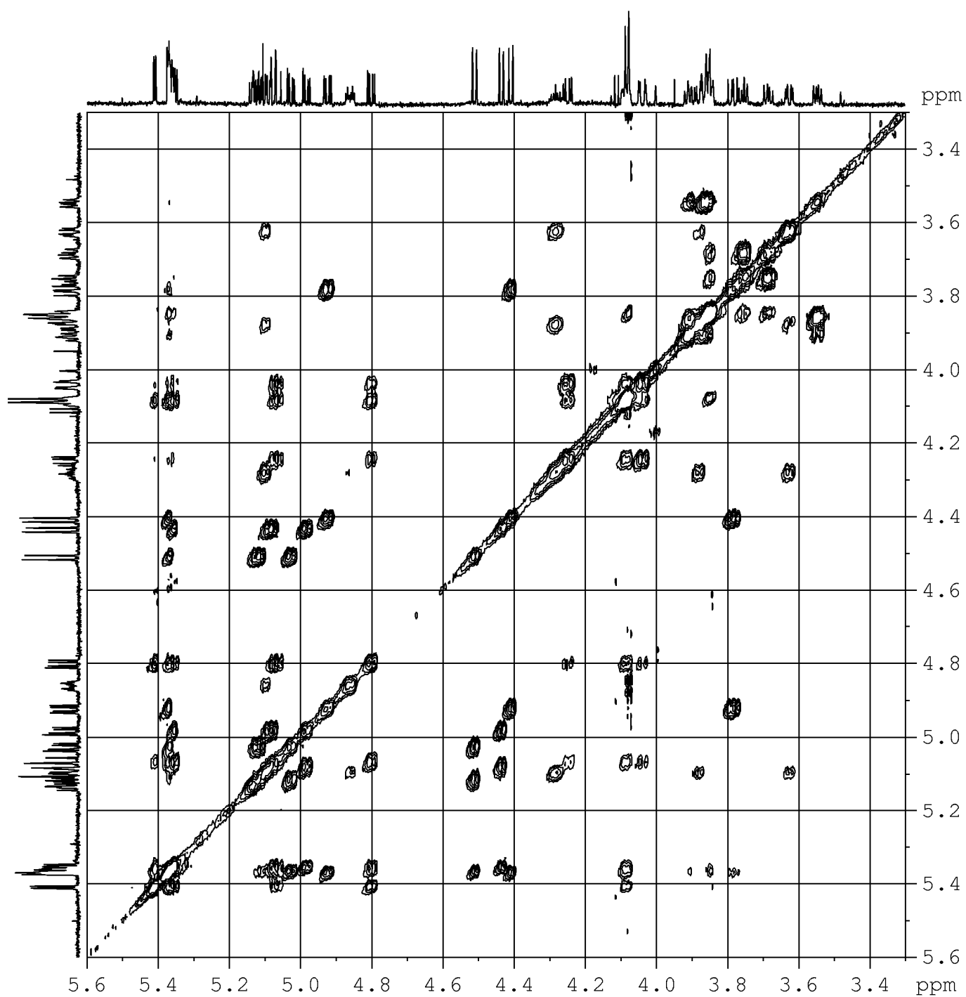
TOCSY spectrum (700 MHz, CDCl 3 ,) of neurosporide peracetate 1b
