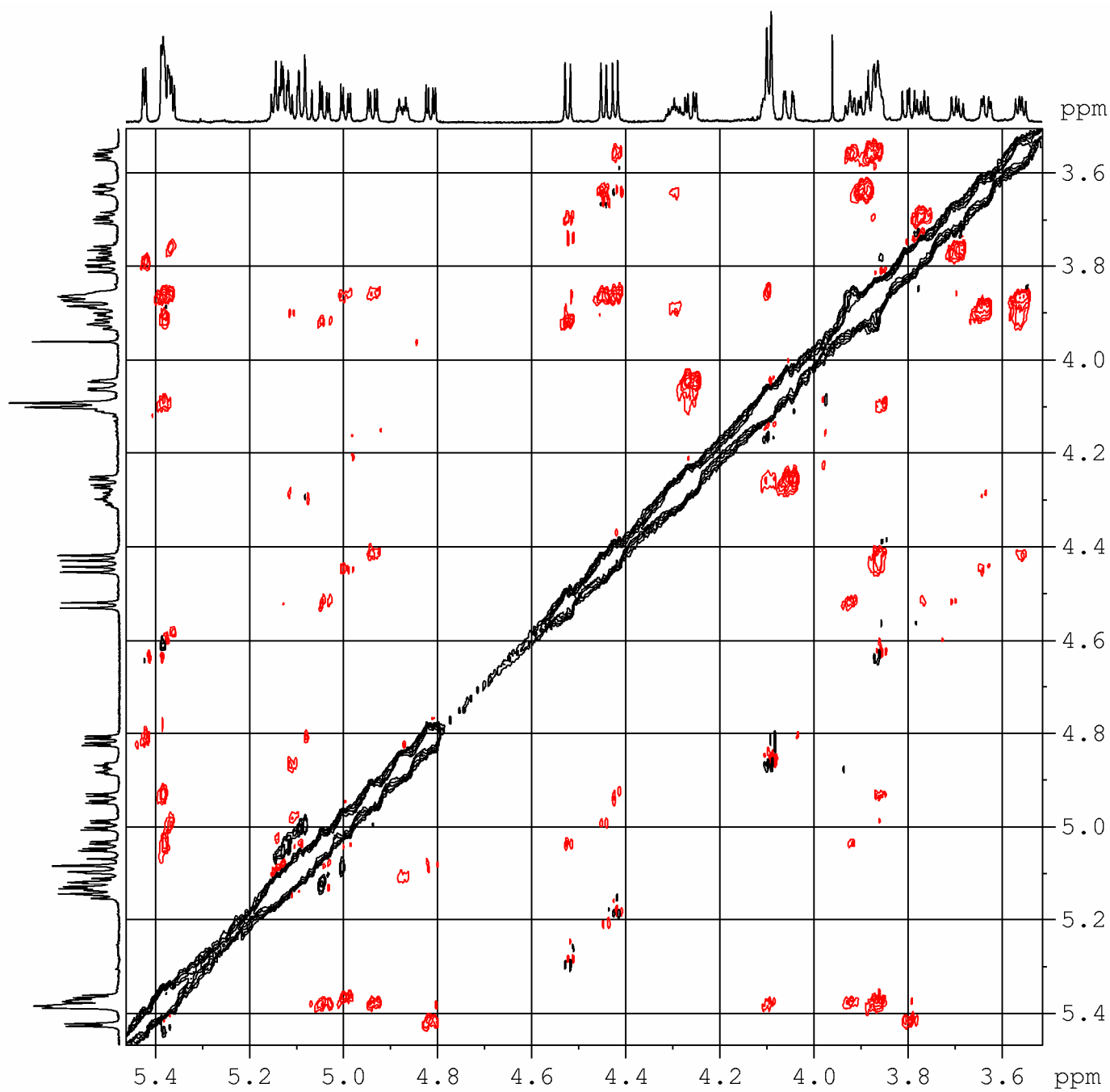
ROESY spectrum (700 MHz, \text{CDCl}_3 ,) of neurosporaside peracetate 1b
