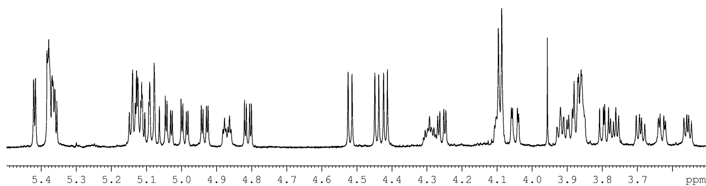
1 H NMR spectrum (700 MHz, CDCl 3 ) of neurosporaside peracetate 1b (mid-field expansion)
