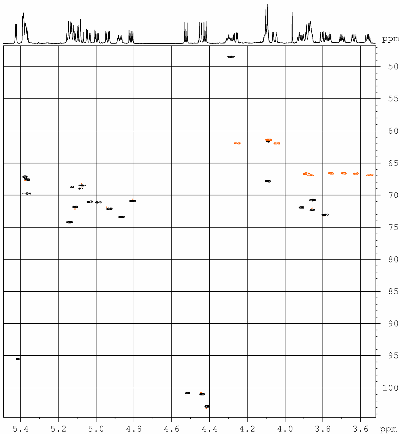
HSQC spectrum (700 MHz, CDCl 3 ) of neurosporaside peracetate 1b
