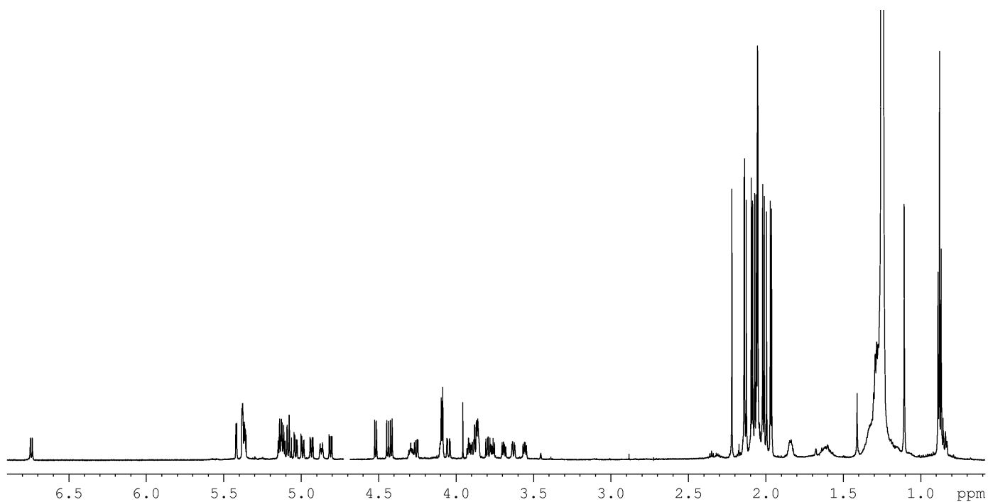
1 H NMR spectrum (700 MHz, CDCl 3 ) of neurosporaside peracetate 1b
