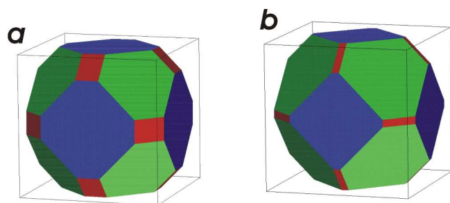
Figure S3: Wulff shapes of dry (a) and partially hydroxylated (b) \text{Co}_3\text{O}_4 (exposed planes are colored as: blue – (100), red – (110), green – (111)); for other shapes see our paper entitled “Periodic DFT and Atomistic Thermodynamic Studies of Cobalt Spinel Nanocrystals in Wet Environment – Molecular Interpretation of Water Adsorption Equilibria”; recently published in J. Phys. Chem. C 2010 , 114 , 22245.
