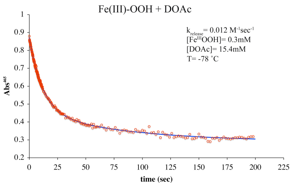
Figure S-24. Kinetics of deuterated acetic acid-induced release of H 2 O 2 from [Fe III (S Me2 N 4 (tren))(OOH)] + ( 2 ) to afford [Fe III (S Me2 N 4 (tren))(O(H)Me)] + ( 4 ) in MeOH at -78 °C.
