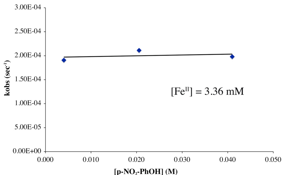
Figure S-18. k_{\text{obs}} vs [\text{p-NO}_2\text{-PhOH}] plot showing zero order dependence on proton donor when [\text{Fe}^{\text{III}}(\text{S}^{\text{Me}_2}\text{N}_4(\text{tren}))(\text{OOH})]^+ ( 2 ) formation occurs in the presence of acids strong enough to convert \text{O}_2^- to \text{HO}_2 .
