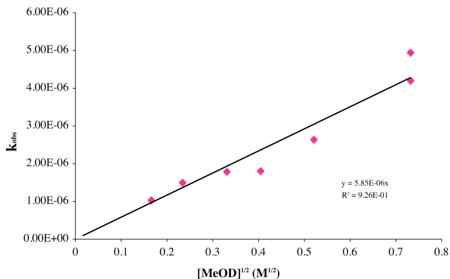
Figure S-6. k_{\text{obs}} vs [\text{HA}]^{1/2} plot for proton donor \text{HA} = \text{MeOD} -induced [\text{Fe}^{\text{III}}(\text{S}^{\text{Me}_2}\text{N}_4(\text{tren}))(\text{OOH})]^+ ( 2 ) formation in THF at -78^\circ\text{C} . [\text{O}_2^-] = 0.35\text{ mM} , [\text{Fe}^{\text{II}}] = 6.5\text{ mM} .
