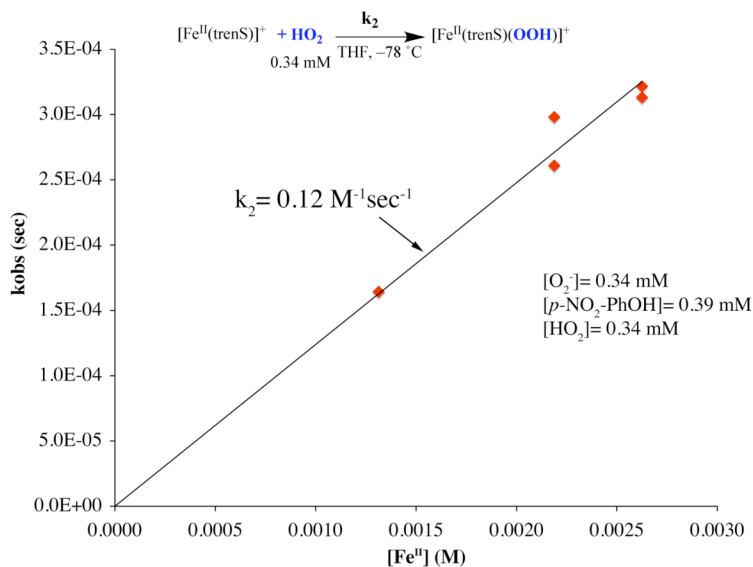
Figure S-16. k_{\text{obs}} vs [\text{Fe}^{\text{II}}] plot for a proton donor (HA = p-NO 2 -PhOH) strong enough to completely convert O 2 - to HO 2 . Under these conditions, (i.e., when [\text{HO}_2] = [\text{O}_2^-] ) the rate expression simplifies to the second order expression shown in equation (2), and the rate constant k_2 can be obtained directly from the slope.
