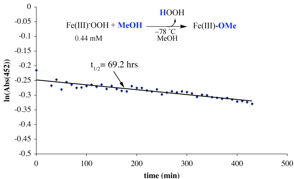
Figure S-20. Kinetics of methanol-induced conversion of [\text{Fe}^{\text{III}}(\text{S}^{\text{Me}_2}\text{N}_4(\text{tren}))(\text{OOH})]^+ ( 2 ) to [\text{Fe}^{\text{III}}(\text{S}^{\text{Me}_2}\text{N}_4(\text{tren}))(\text{OMe})]^+ ( 3 ) in MeOH at -78^\circ\text{C} .
