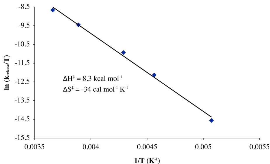
Figure 23. Eyring plot for AcOH-induced release of H 2 O 2 from hydroperoxo [Fe III (S Me2 N 4 (tren))(OOH)] + ( 2 ) to afford methanol-bound [Fe III (S Me2 N 4 (tren))(O(H)Me)] + ( 4 ).
