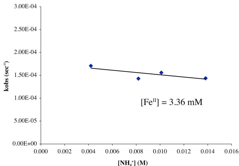
Figure S-19. k_{\text{obs}} vs [\text{NH}_4^+] plot showing zero order dependence on proton donor when [\text{Fe}^{\text{III}}(\text{S}^{\text{Me}_2}\text{N}_4(\text{tren}))(\text{OOH})]^+ ( 2 ) formation occurs in the presence of acids strong enough to convert \text{O}_2^- to \text{HO}_2 .
