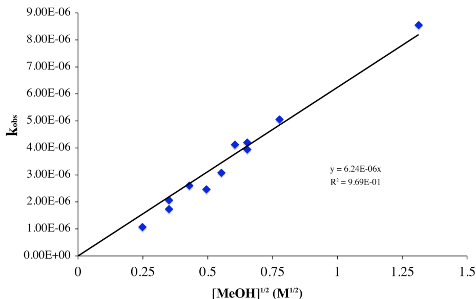
Figure S-5. k_{\text{obs}} vs [\text{HA}]^{1/2} plot for proton donor \text{HA} = \text{MeOH} -induced [\text{Fe}^{\text{III}}(\text{S}^{\text{Me}_2}\text{N}_4(\text{tren}))(\text{OOH})]^+ ( 2 ) formation in THF at -78^\circ\text{C} . [\text{O}_2^-] = 0.35\text{ mM} , [\text{Fe}^{\text{II}}] = 6.5\text{ mM} .
