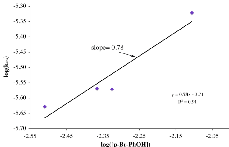
Figure S-15. Determination of the reaction order (half) with respect to HA = p-Br-PhOH, using a \log(k_{\text{obs}}) vs \log([HA]) plot, for the proton-assisted formation of [\text{Fe}^{\text{III}}(\text{S}^{\text{Me}_2}\text{N}_4(\text{tren}))(\text{OOH})]^+ ( 2 ) from [\text{Fe}^{\text{II}}(\text{S}^{\text{Me}_2}\text{N}_4(\text{tren}))]^+ ( 1 ) + (18-crown-6-K + )(O 2 - ) in THF at -78 °C. [O 2 - ] = 0.35 mM, [Fe II ] = 6.5 mM.
