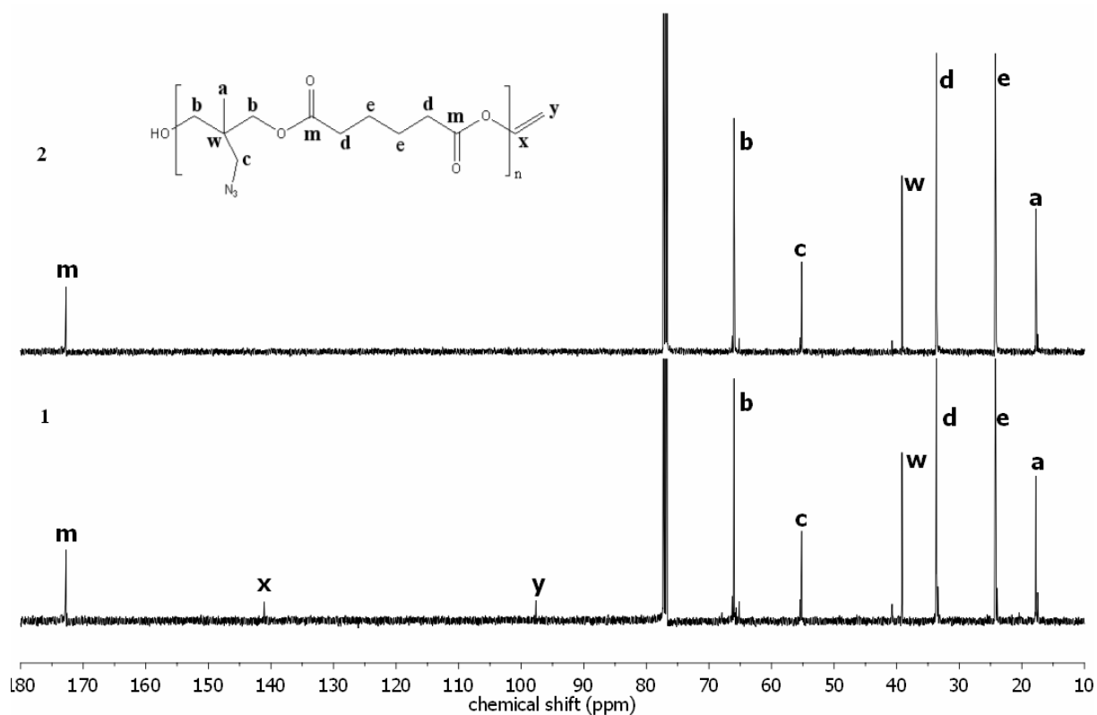
Supplementary Figure 2. ^{13}\text{C} NMR spectra of PAA in \text{CDCl}_3 polymerized for 20h (1, lower graph), and for 3 days (2, upper graph).
