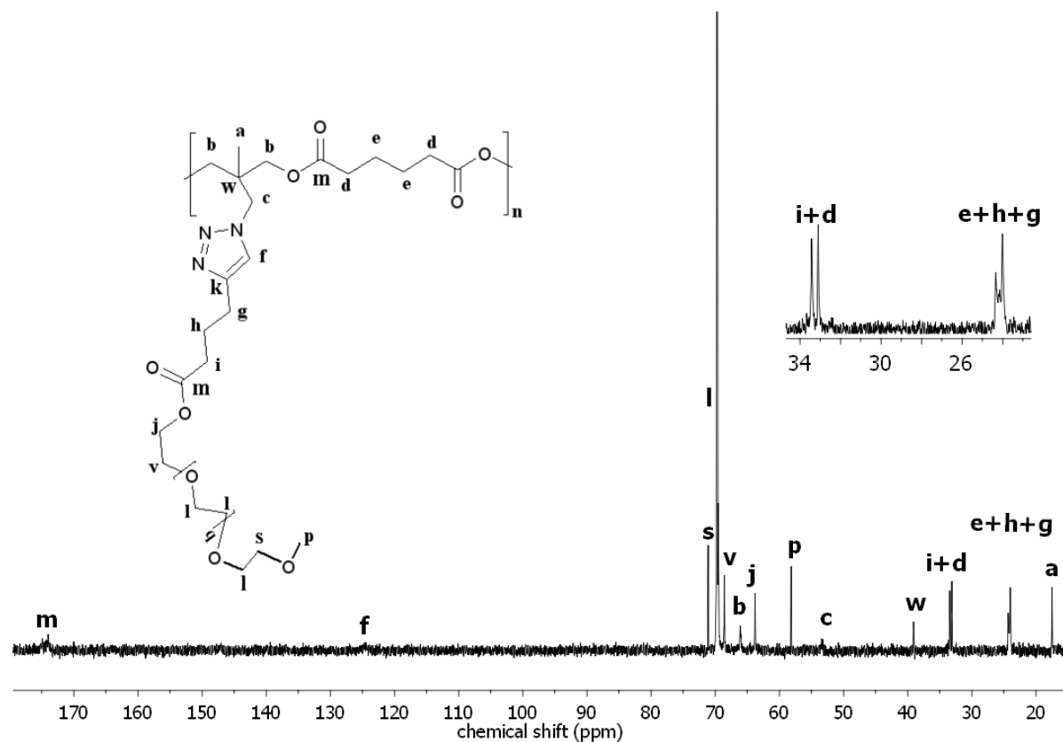
Supplementary Figure 3: ^{13}\text{C} NMR spectrum of PAA-g-PEO in \text{D}_2\text{O} .
