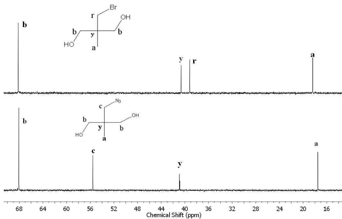
Supplementary Figure 1: ^{13}\text{C} NMR spectra of 2-(bromomethyl)-2-methylpropane-1,3-diol and 2-(azidomethyl)-2-methylpropane-1,3-diol (AMD).
