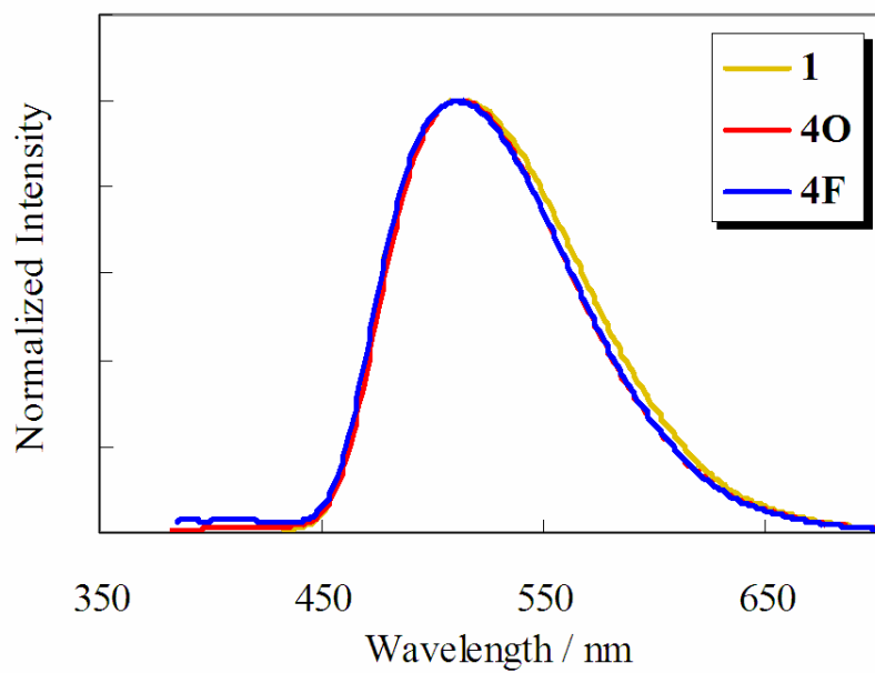
Figure S1. Normalized emission spectra of polymers and model compound in \text{CHCl}_3 ( 1.0 \times 10^{-5} M).
