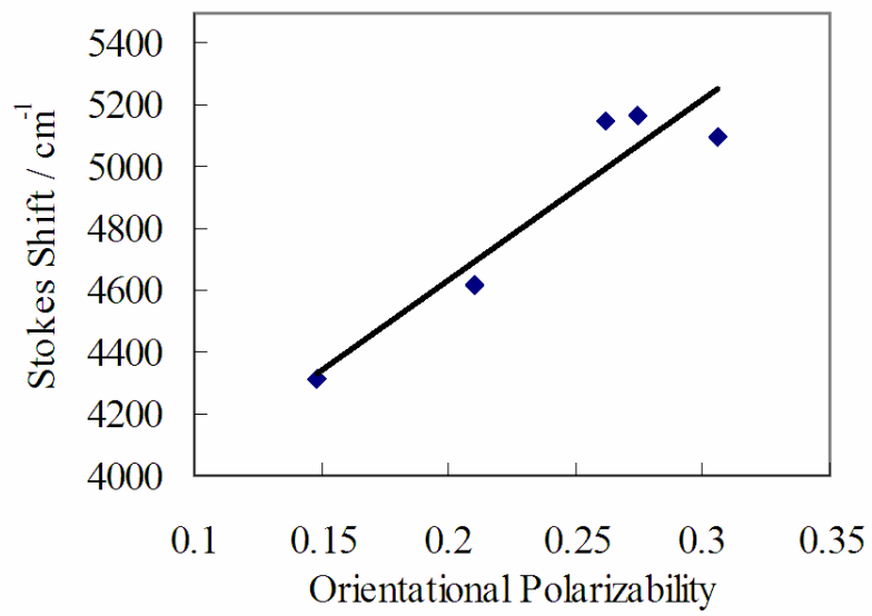
Figure S2. Lippert plot of model compound 1.
