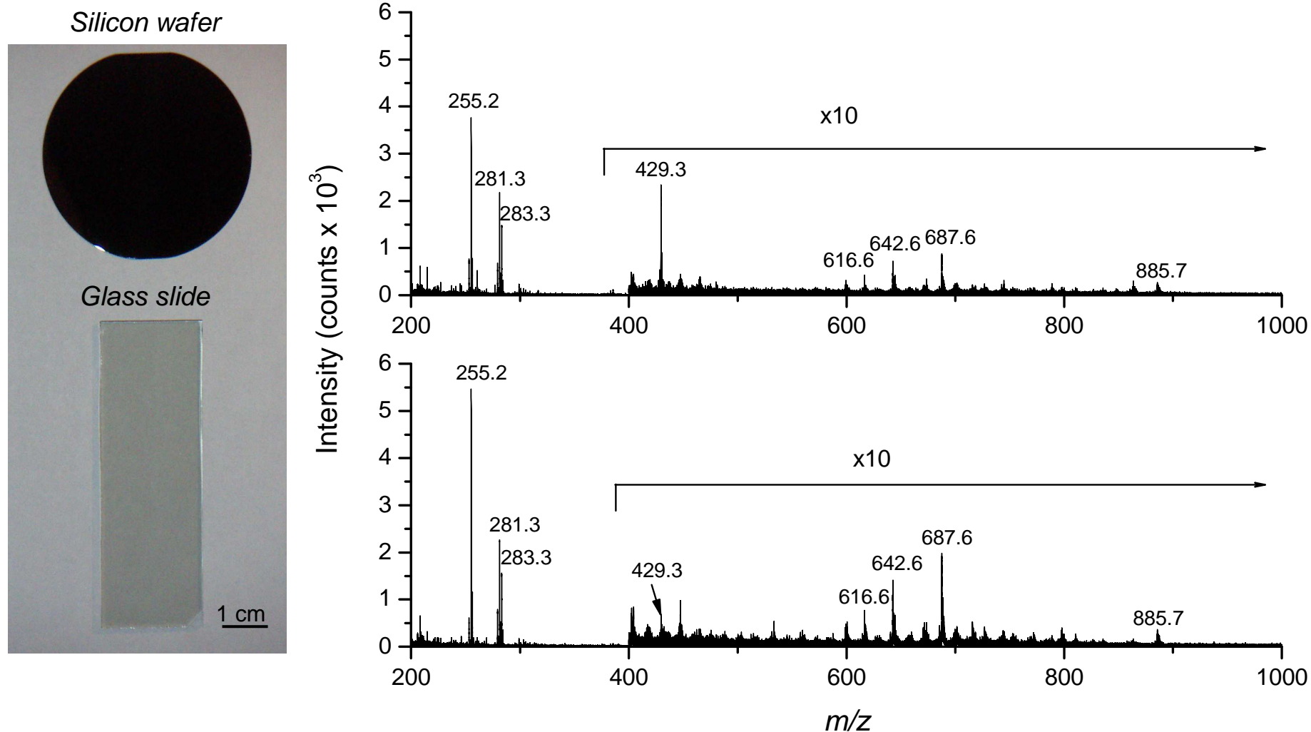
Figure S-1. Negative ion ToF-SIMS mass spectra on silicon wafer or gold coated glass slide. ToF-SIMS acquisitions were performed on serial tissue sections from liver cirrhosis deposited on silicon wafer or gold coated glass slide. Similar spectra were observed in terms of sensitivity and resolution on the two sample holders.
