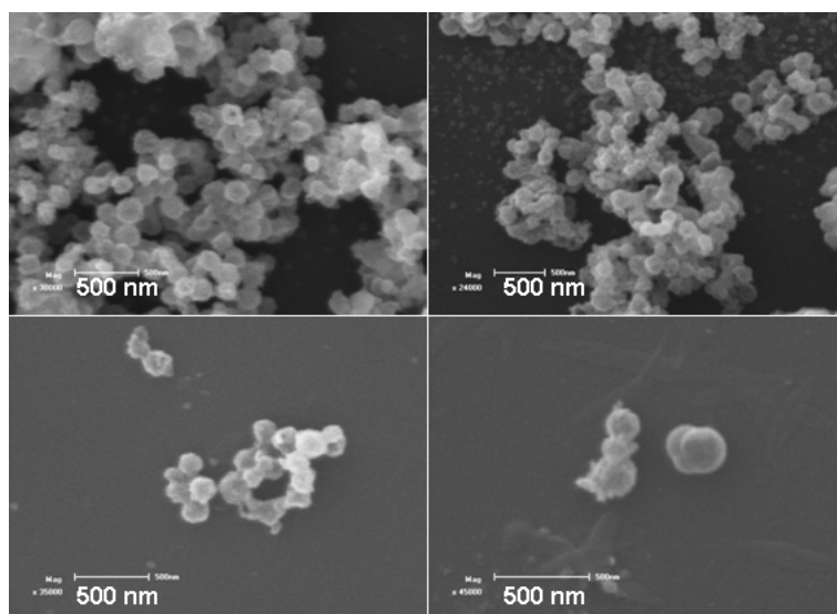
Figure S1. SEM images of the polypyrrole coated SnO 2 hollow spheres.
