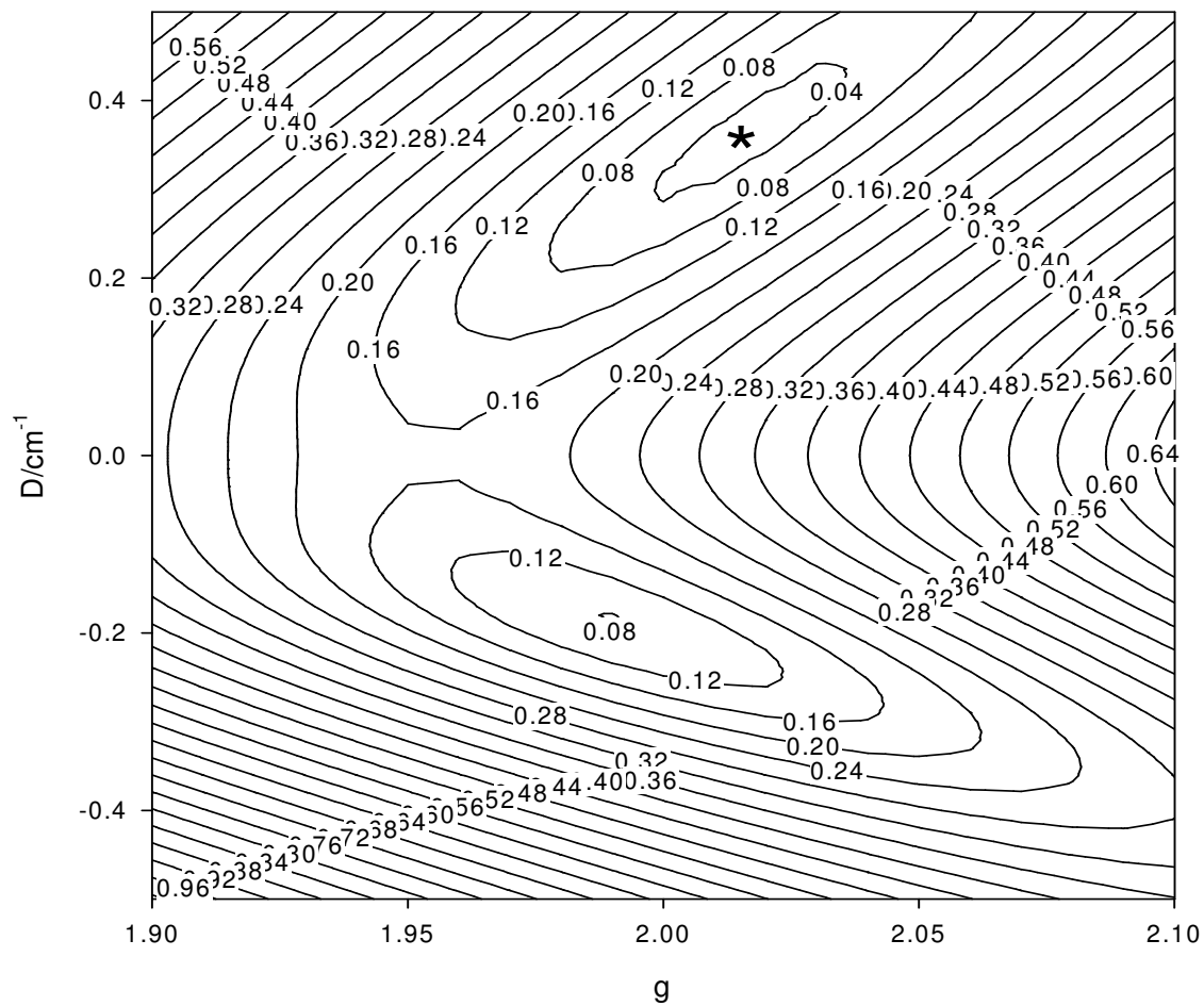
Figure S4. Two-dimensional contour plot of the fitting error surface vs D and g for 4\cdot\text{H}_2\text{O}
