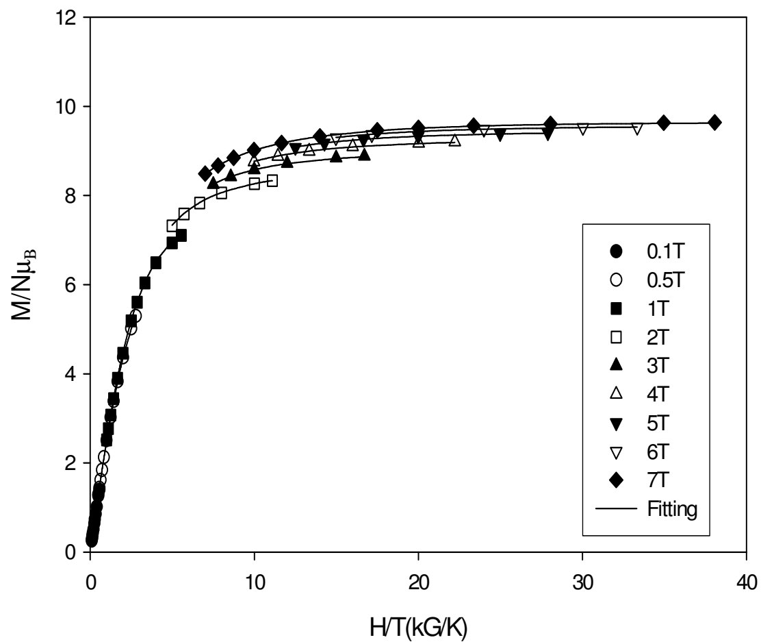
Figure S1. Plot of reduced magnetization ( M/N\mu_B ) vs H/T for complex 3\cdot H_2O . The solid lines are the fit of the data; see the text for the fit parameters.
