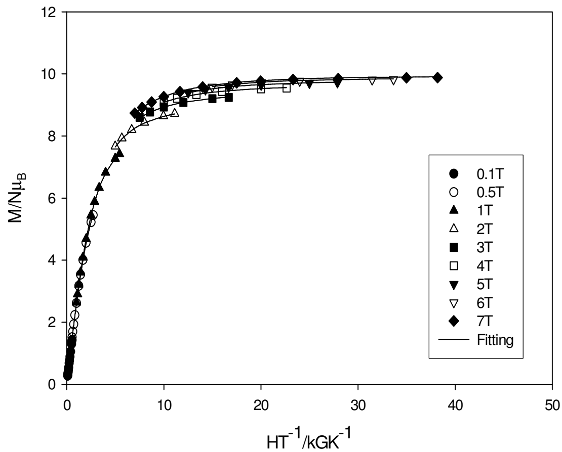
Figure S3. Plot of reduced magnetization ( M/N\mu_B ) vs H/T for complex 4\cdot H_2O . The solid lines are the fit of the data; see the text for the fit parameters.
