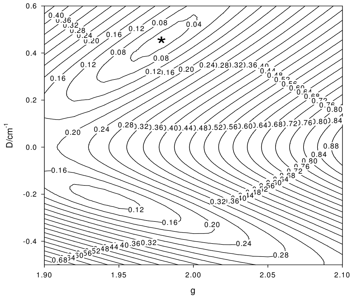
Figure S2. Two-dimensional contour plot of the fitting error surface vs D and g for 3·H 2 O
