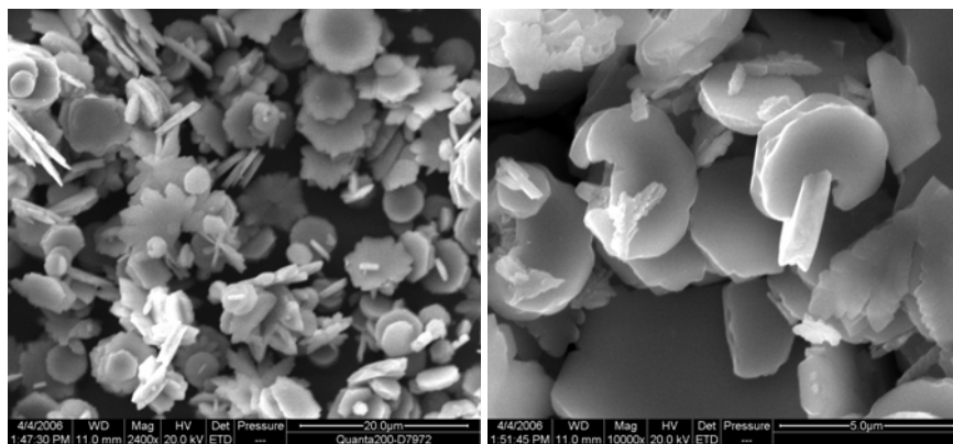
Figure 1 SEM images of \alpha -Fe 2 O 3 crystal obtained with [Fe(CN) 6 ] 3- /NaOH molar ratio of 1/3.5.
