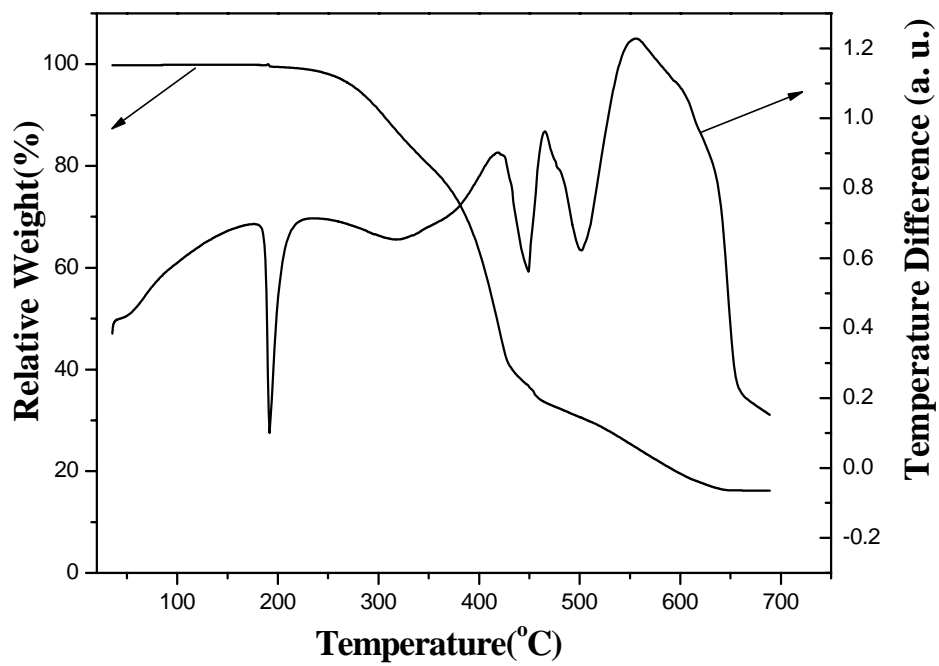
Supporting Figure TGA-DTA curve of Dy(PM) 3 (TP) 2
