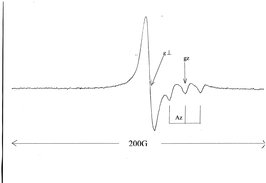
Supporting Figure 2. Q-band powder-pattern ESR spectrum of the phenoxyl radical derivative generated from a novel probe, \alpha -(3, 5-di- tert -butyl-4-hydroxyphenyl)- N-tert -butylnitron
