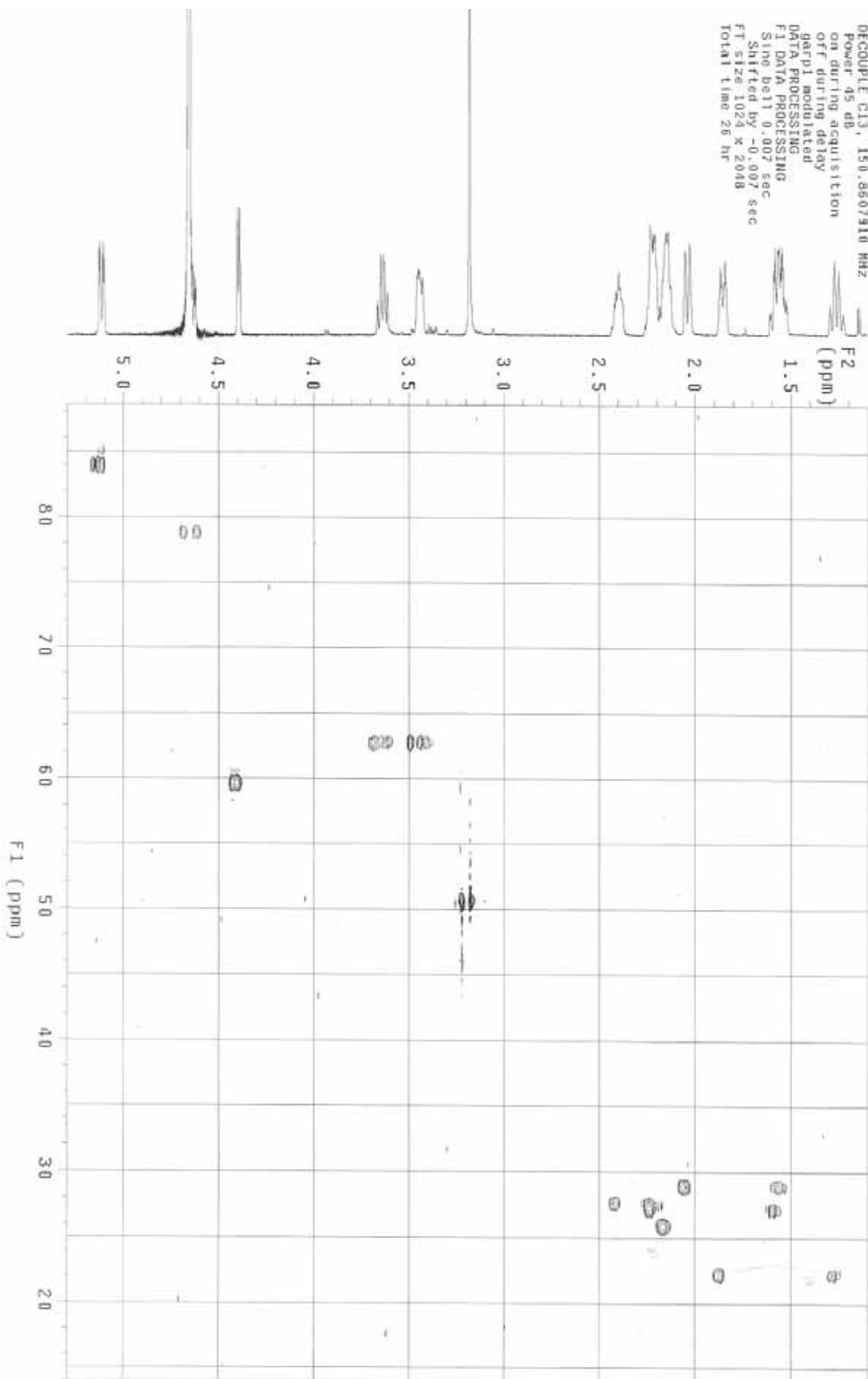
FigS. 3. HMQC for 1.
