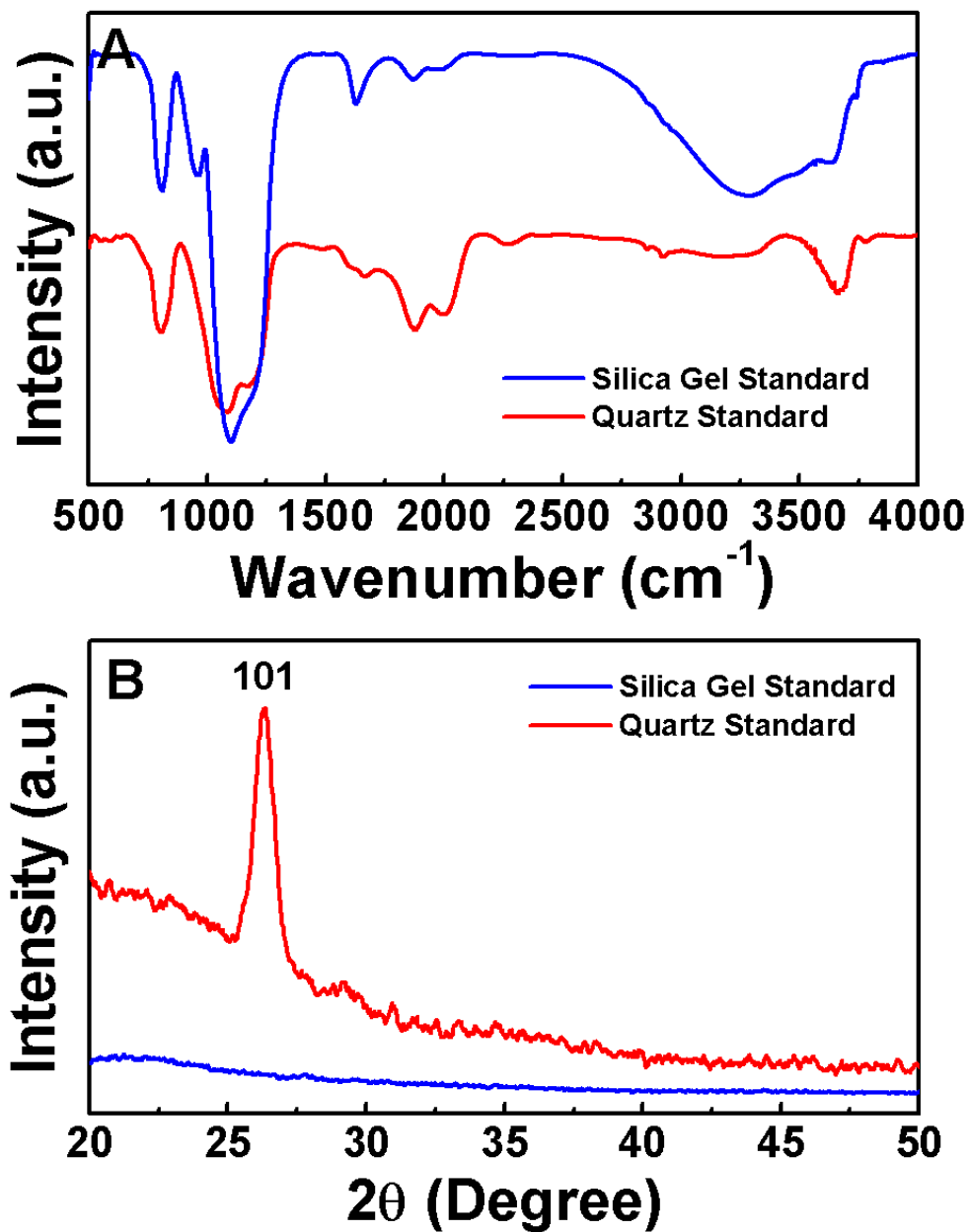
S3. A) FTIR spectra recorded from standard silica gel and quartz particles; B) XRD patterns recorded from standard silica gel and quartz particles.
