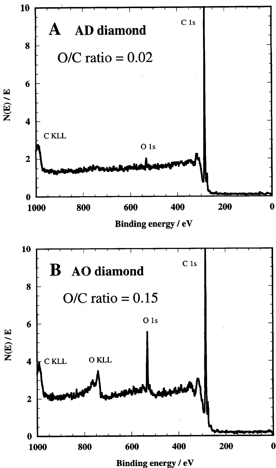
Figure S1. Survey X-ray photoelectron spectra for (A) AD diamond and (B) AO diamond. The source of X-ray was Mg- K_{\alpha} .
