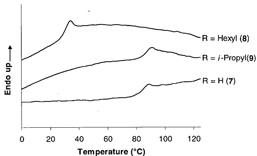
Figure S1. DSC traces for polymers 7-9.
