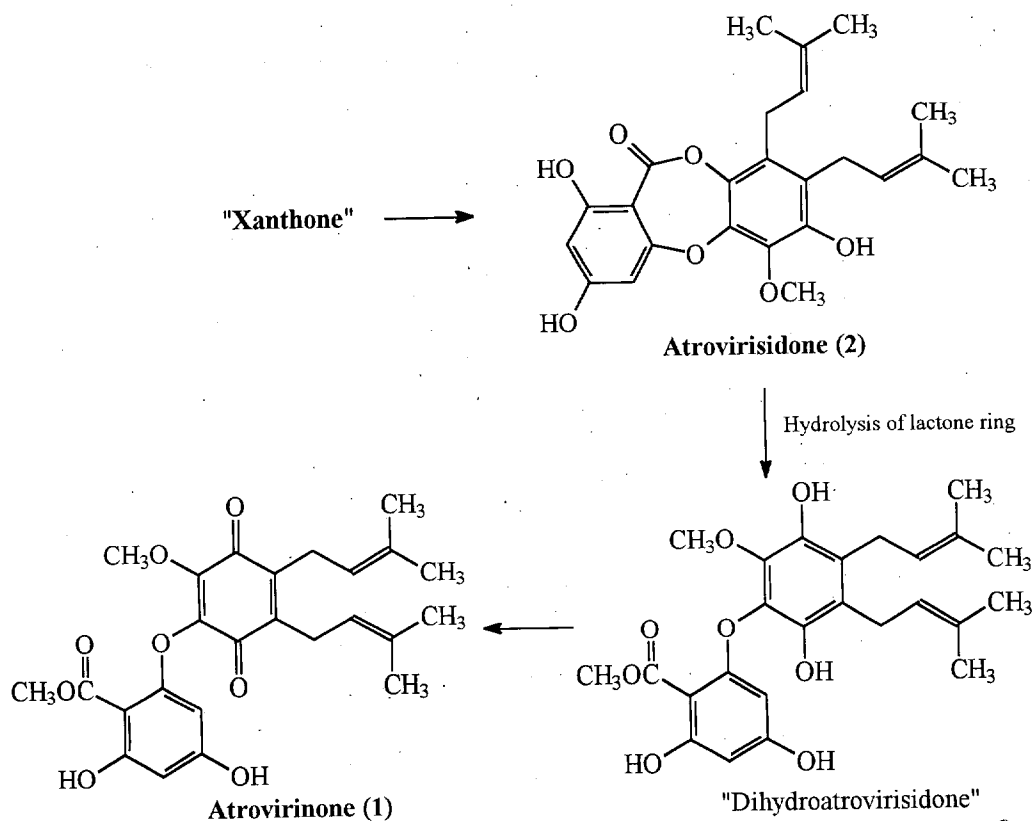
Scheme 1. Postulated biogenetic relationship of atrovirinone (1) and atrovirisidone (2).
