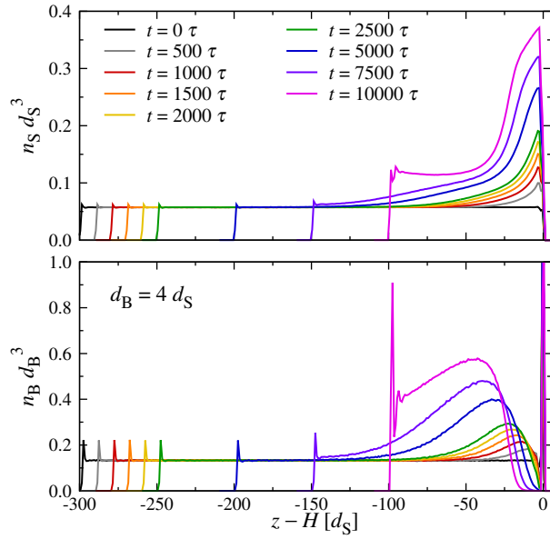
Figure S2: Number density profiles during drying for d_B = 4 d_S and v = 0.02 d_S/\tau .
