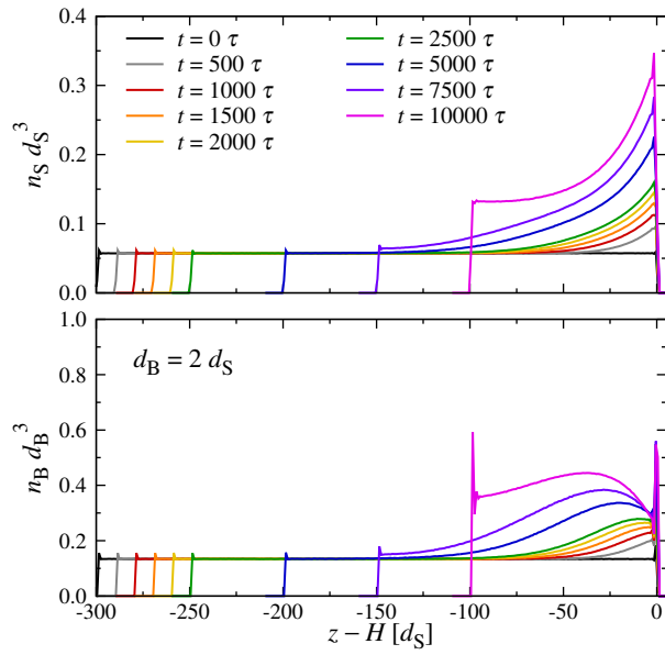
Figure S3: Number density profiles during drying for d_B = 2 d_S and v = 0.02 d_S/\tau .
