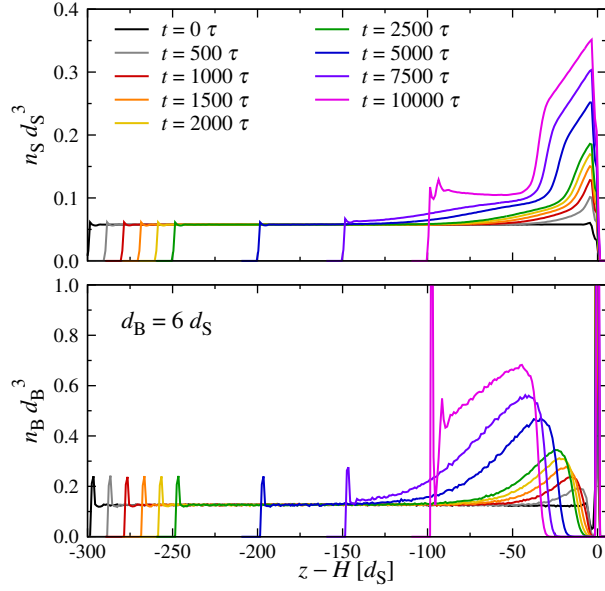
Figure S1: Number density profiles during drying for d_B = 6 d_S and v = 0.02 d_S/\tau .
