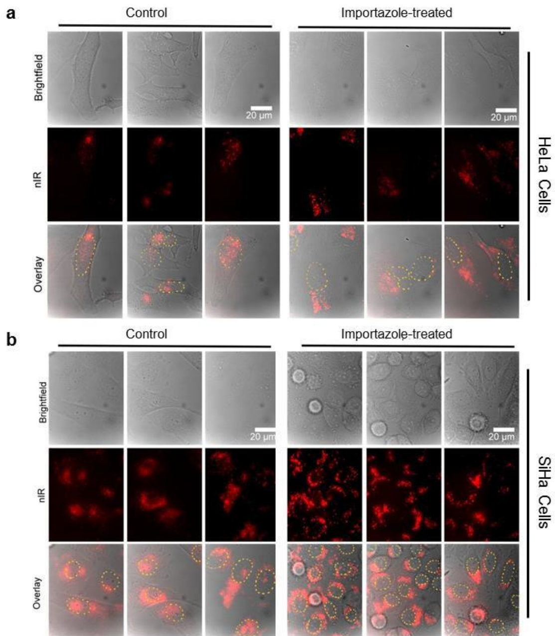
Figure S9. Near-infrared emission of guanidinium-nanotube complexes introduced after adding importazole to the cell culture media. a , HeLa cells. b , SiHa cells. Cell nuclei are outlined with dotted yellow lines.
