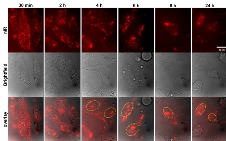
Figure S5. Time-course images of guanidinium-nanotube complex near-infrared emission in HeLa cells. Cell nuclei are outlined with dotted yellow lines.
