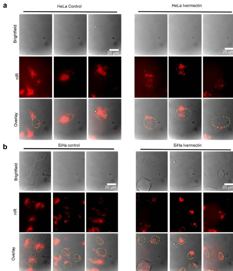
Figure S8. Near-infrared emission of guanidinium-nanotube complexes introduced after adding ivermectin to the cell media. a , HeLa cells. b , SiHa cells. Cell nuclei are outlined with dotted yellow lines.
