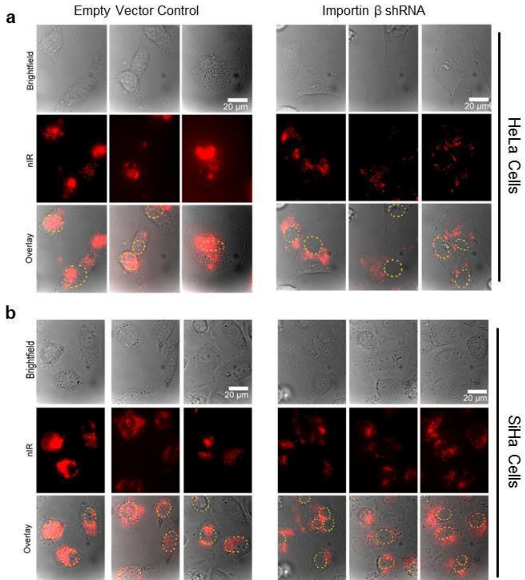
Figure S10. Near-infrared emission of guanidinium-nanotube complexes introduced after knockdown of importin \beta using shRNA. a , HeLa cells. b , SiHa cells. Cell nuclei are outlined with dotted yellow lines.
