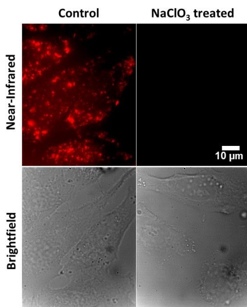
Figure S6. Near-infrared emission from guanidinium-nanotube complexes in HeLa cells treated with \text{NaClO}_3 before introducing the complexes.
