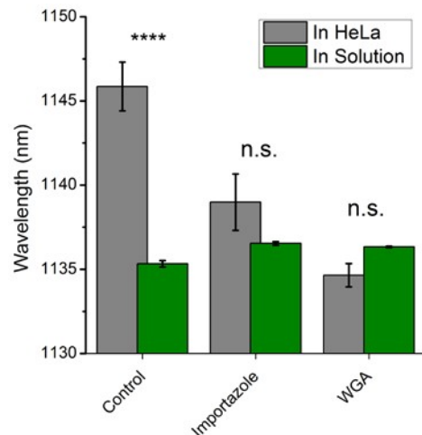
Figure S11. Comparisons of carbon nanotube emission wavelength in HeLa cells and under cell-free conditions (in aqueous solution) with inhibitors of nuclear translocation. Graphs represent mean \pm standard deviation from 3 replicate experiments. **** P < 0.0001 ( P < 0.05 significant).
