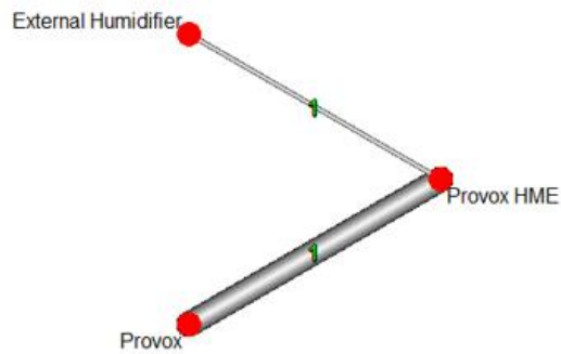
Supplemental Figure S16. Network meta-analysis for Loosening of adhesive of each device.
