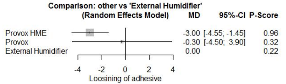
Supplemental Figure S16. Network meta-analysis for Loosening of adhesive of each device.
